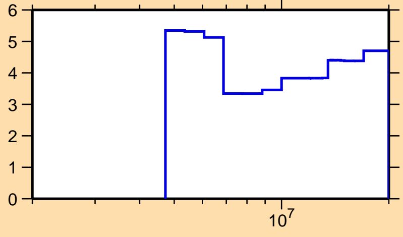
\Delta\sigma/\sigma vs. E for ^{22}\text{O}(n,\text{nonel.})
