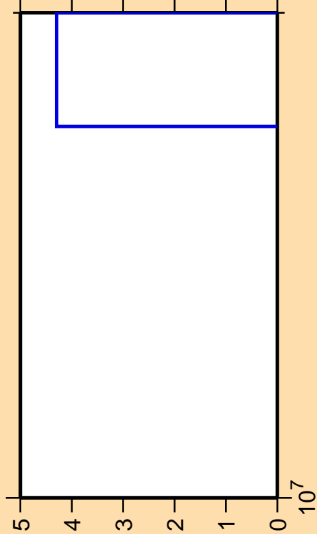
\Delta\sigma/\sigma vs. E for ^{22}\text{O}(n,n\alpha)
