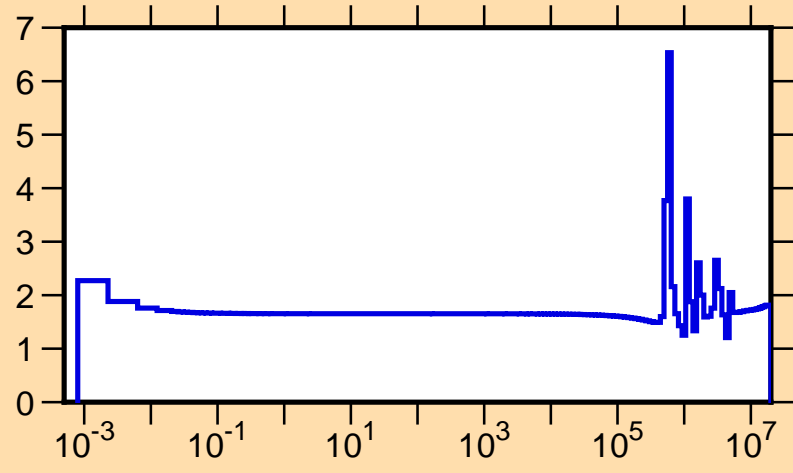
\sigma vs. E for ^{22}\text{O}(n,\text{tot.})
