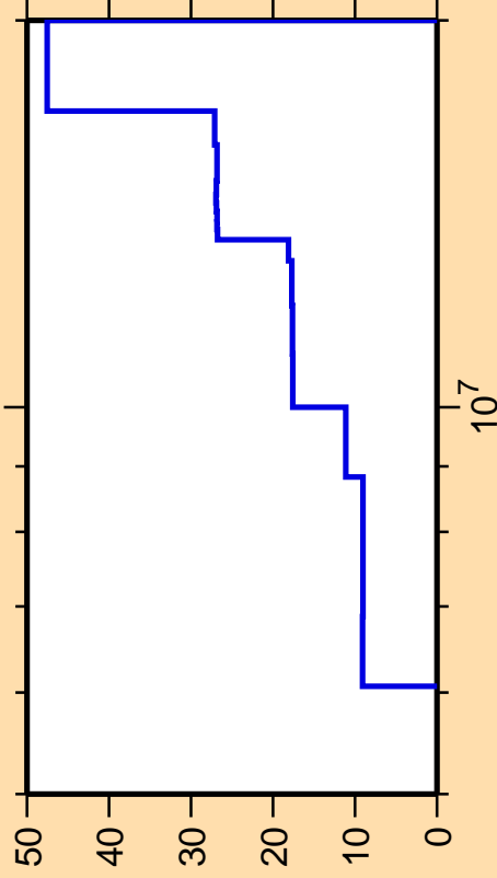
\Delta\sigma/\sigma vs. E for ^{22}\text{O}(n,n_4)
