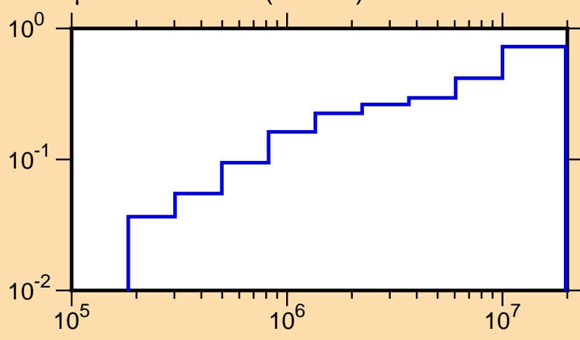
\mu vs. E for ^{22}\text{O}(\text{mt251})
