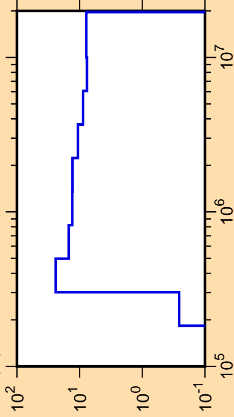
\Delta\mu/\mu vs. E for ^{22}\text{O}(\text{mt251})
