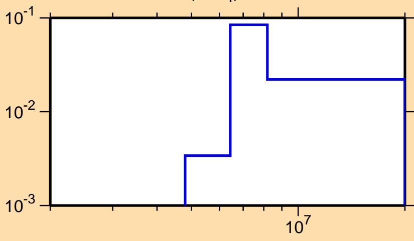
\sigma vs. E for ^{22}\text{O}(n,n_4)
