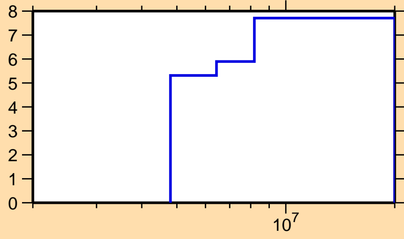
\Delta\sigma/\sigma vs. E for ^{22}\text{O}(n,\text{inel.})
