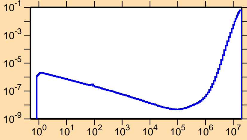
\sigma vs. E for ^{168}\text{Os}(n,p\alpha)
