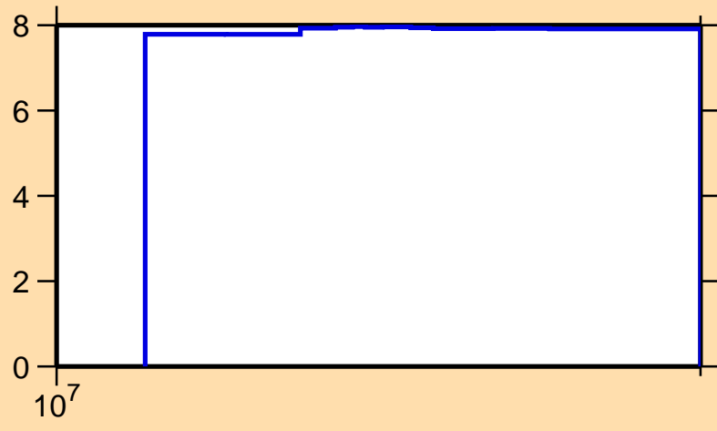
\Delta\sigma/\sigma vs. E for ^{168}\text{Os}(n,\text{nonel.})
