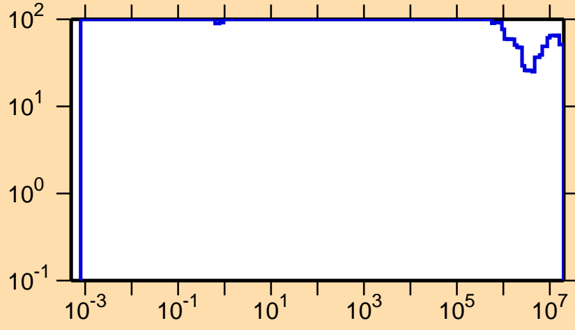
\Delta\sigma/\sigma vs. E for ^{168}\text{Os}(n,p)
