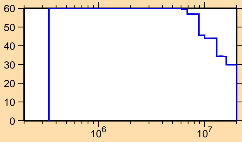
\Delta\sigma/\sigma vs. E for ^{168}\text{Os}(n,\text{inel.})
