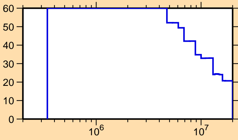
\Delta\sigma/\sigma vs. E for ^{168}\text{Os}(n,n_1)
