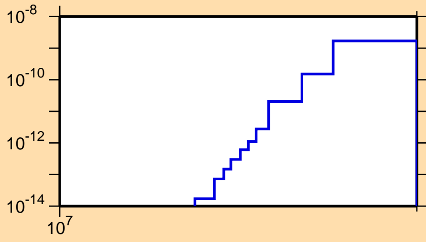
\sigma vs. E for ^{168}\text{Os} (mt 34)
