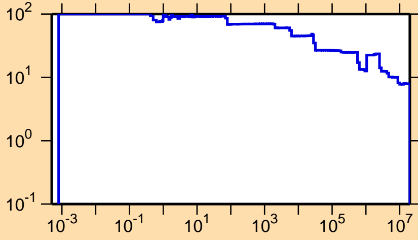
\Delta\sigma/\sigma vs. E for ^{168}\text{Os}(n,\text{nonel.})
