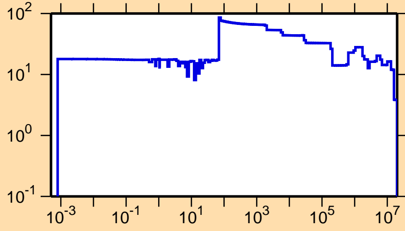
\Delta\sigma/\sigma vs. E for ^{168}\text{Os}(n,\text{el.})
