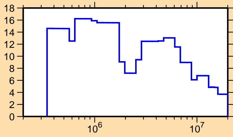
\Delta\sigma/\sigma vs. E for ^{168}\text{Os}(n,\text{tot.})
