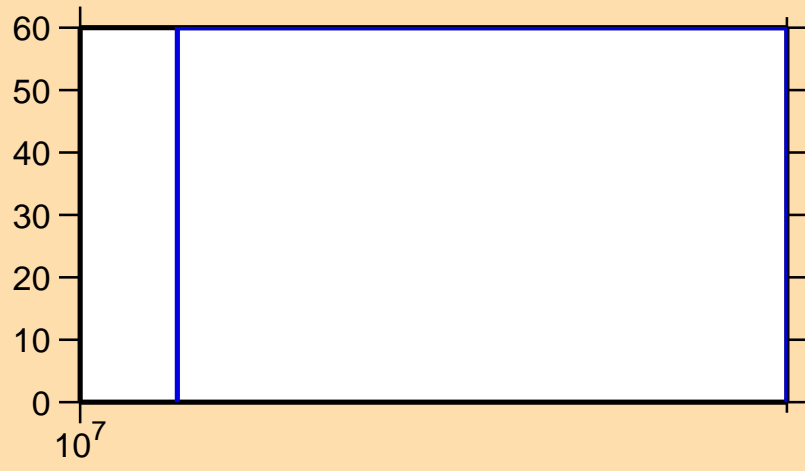
\Delta\sigma/\sigma vs. E for ^{168}\text{Os}(n,2n)
