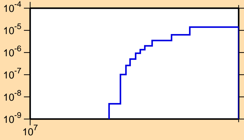
\sigma vs. E for ^{168}\text{Os}(n,2n\alpha)
