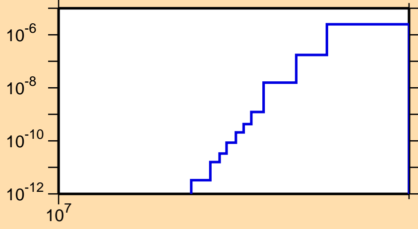
\sigma vs. E for ^{168}\text{Os}(n,\text{pt})
