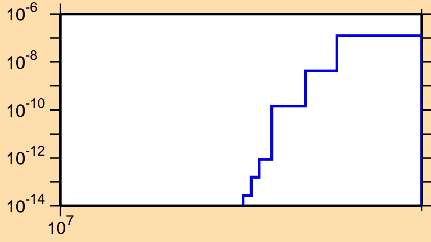
\sigma vs. E for ^{168}\text{Os}(n,\text{nd})
