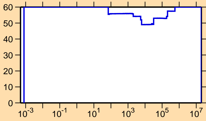
\Delta\sigma/\sigma vs. E for ^{168}\text{Os}(n,\gamma)
