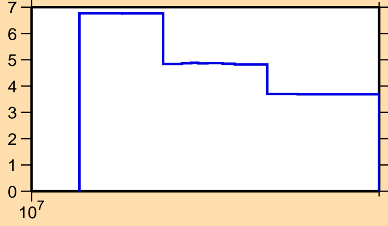
\Delta\sigma/\sigma vs. E for ^{168}\text{Os}(n,\text{tot.})
