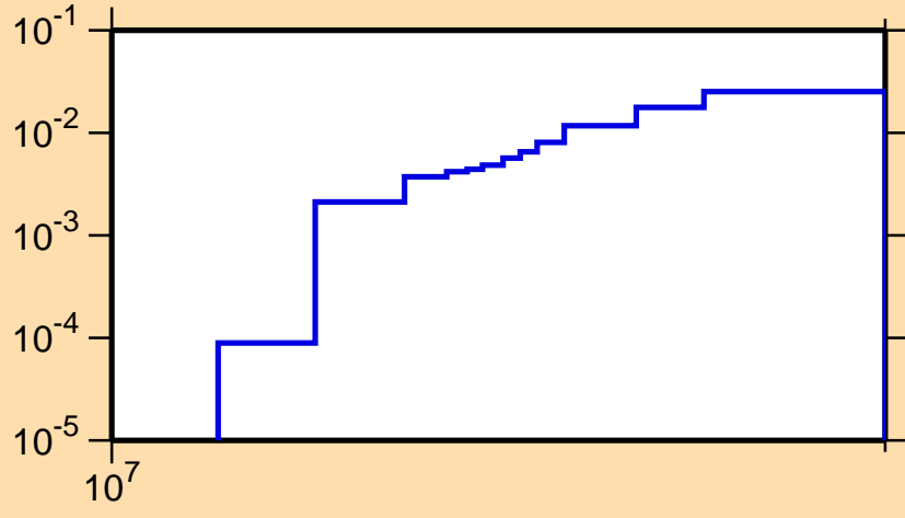
\sigma vs. E for ^{168}\text{Os}(n,2n)
