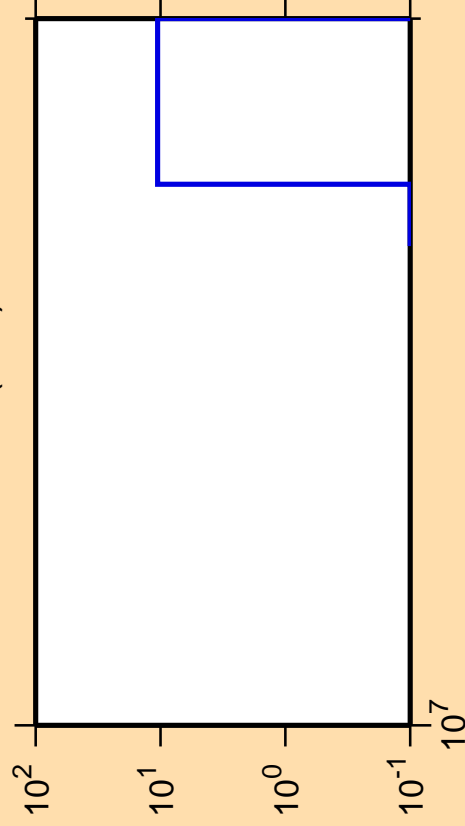
\Delta\sigma/\sigma vs. E for ^{168}\text{Os}(n,nt)
