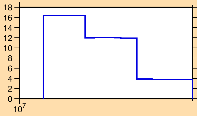
\Delta\sigma/\sigma vs. E for ^{168}\text{Os}(n,\text{el.})
