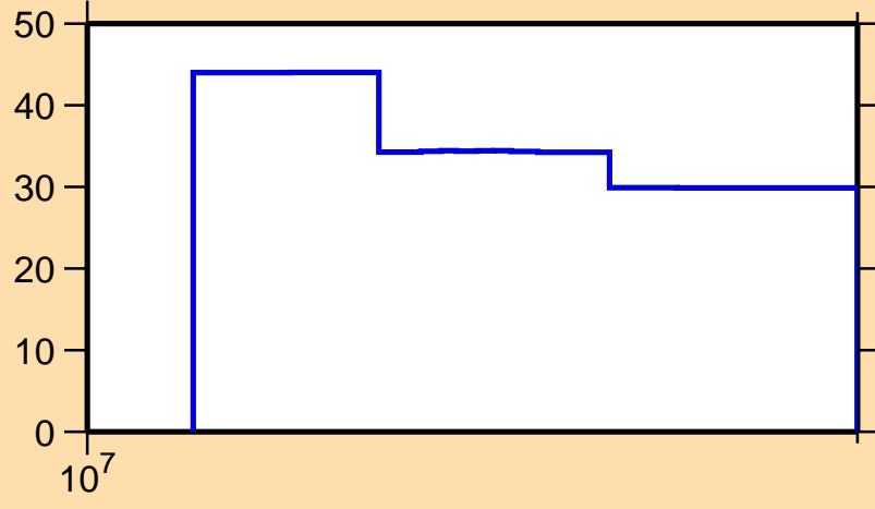
\Delta\sigma/\sigma vs. E for ^{168}\text{Os}(n,\text{inel.})
