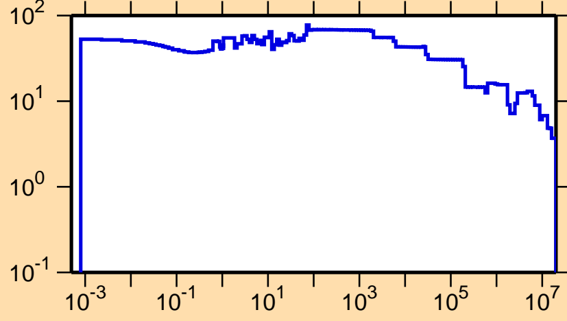
\Delta\sigma/\sigma vs. E for ^{168}\text{Os}(n,\text{tot.})
