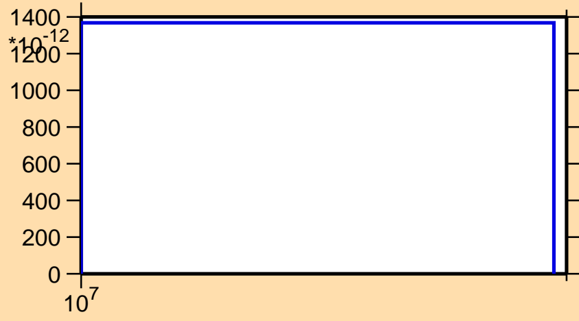
\sigma vs. E for ^{168}\text{Os}(n,\text{nd})
