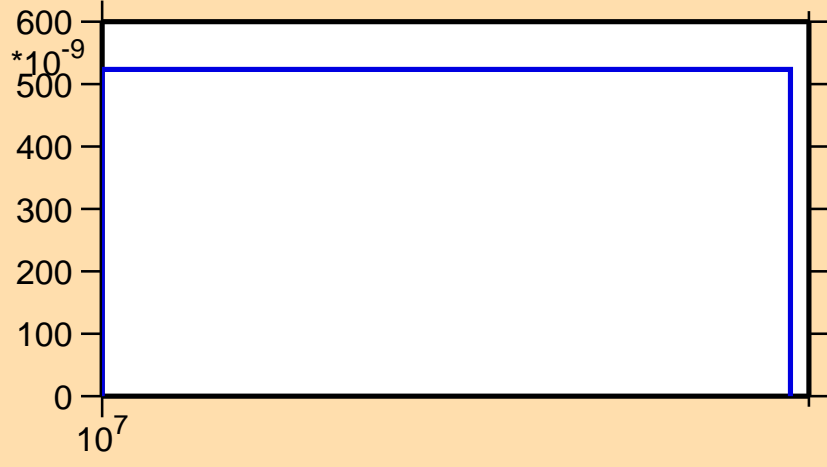
\sigma vs. E for ^{168}\text{Os}(n,2np)
