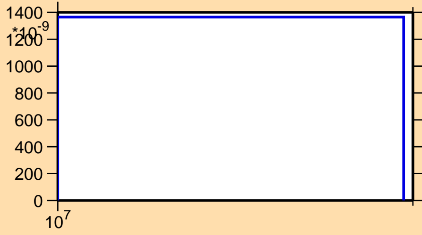
\sigma vs. E for ^{168}\text{Os}(n,2n\alpha)
