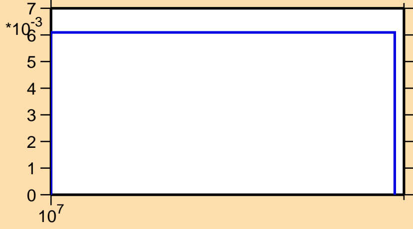
\sigma vs. E for ^{168}\text{Os}(n,2n)
