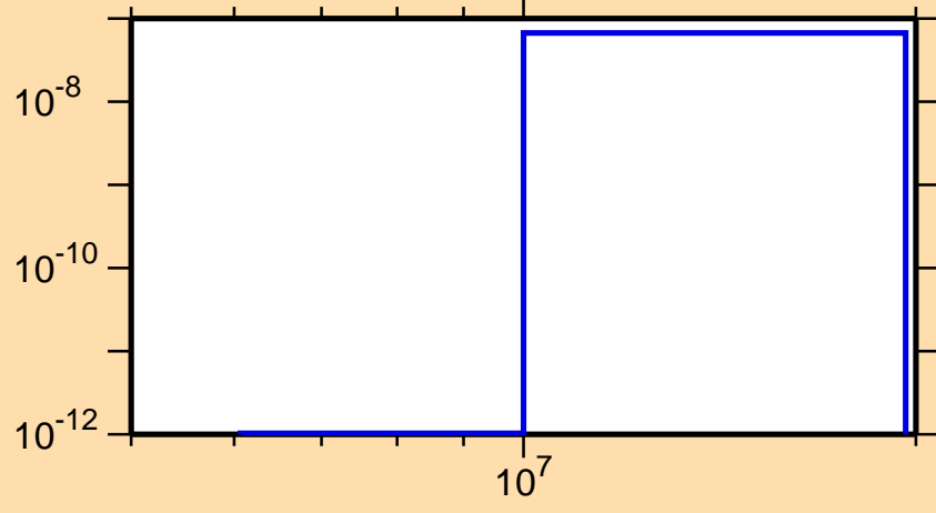
\sigma vs. E for ^{168}\text{Os}(\text{mt117})
