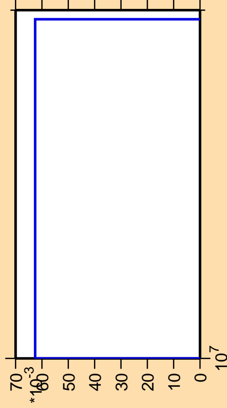
\Delta\sigma/\sigma vs. E for ^{168}\text{Os}(n,nt)
