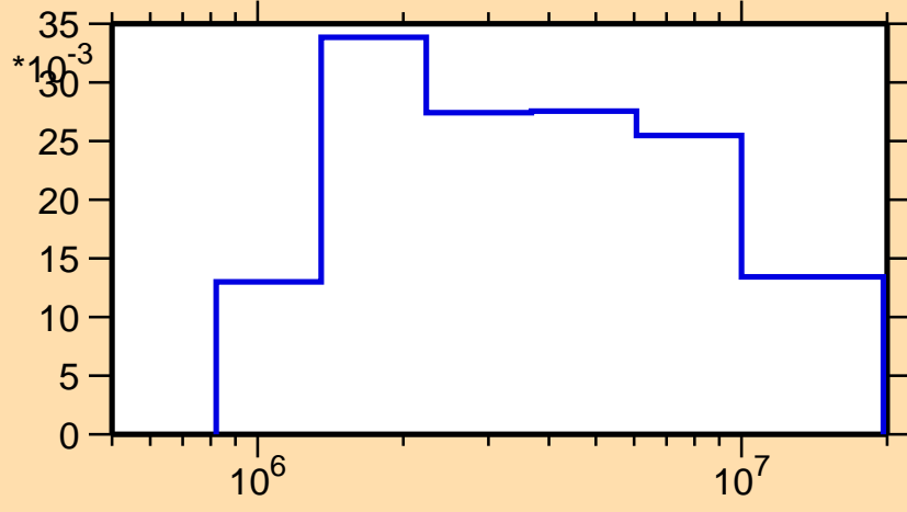
\sigma vs. E for ^{168}\text{Os}(n,n_2)
