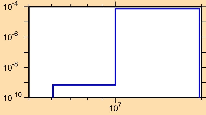
\sigma vs. E for ^{168}\text{Os}(n,\text{pd})
