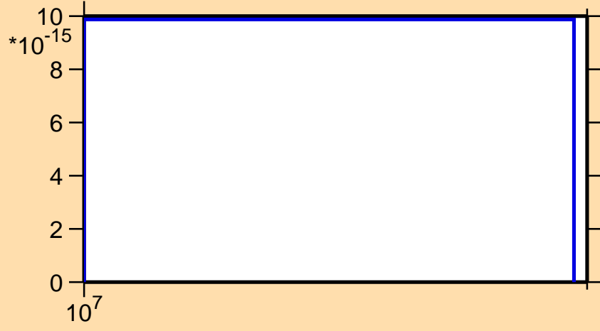
\sigma vs. E for ^{168}\text{Os}(n,nt)
