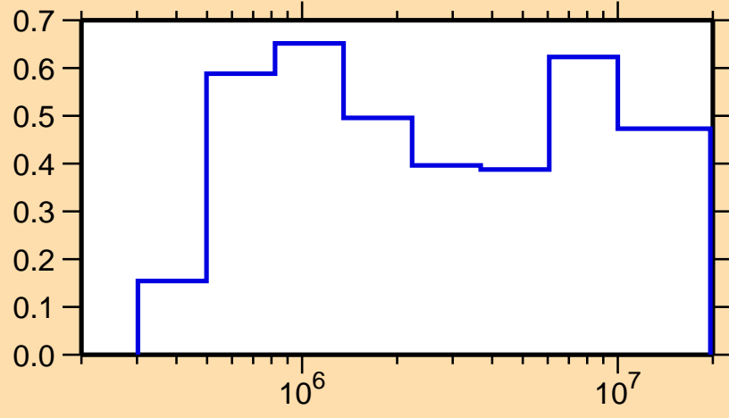
\sigma vs. E for ^{168}\text{Os}(n,\text{inel.})
