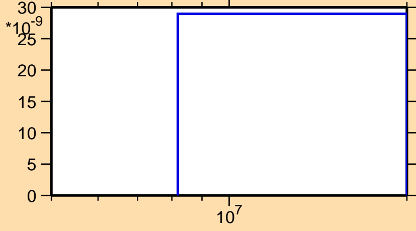
\sigma vs. E for ^{168}\text{Os}(n,pt)
