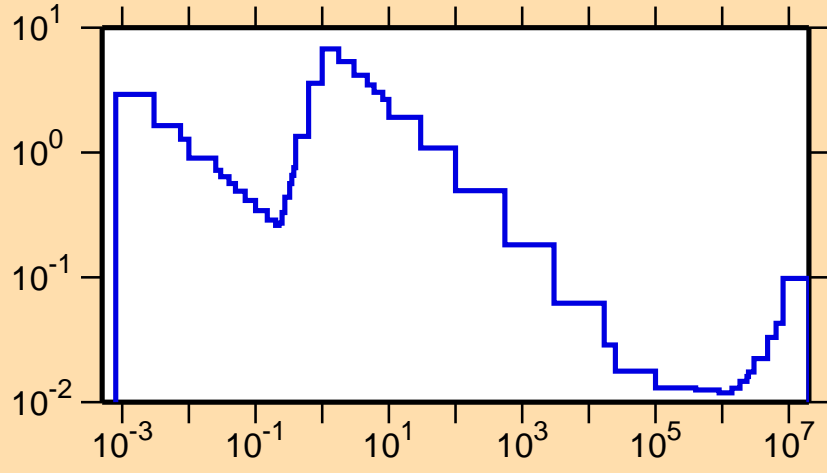
\sigma vs. E for ^{168}\text{Os}(n,\alpha)
