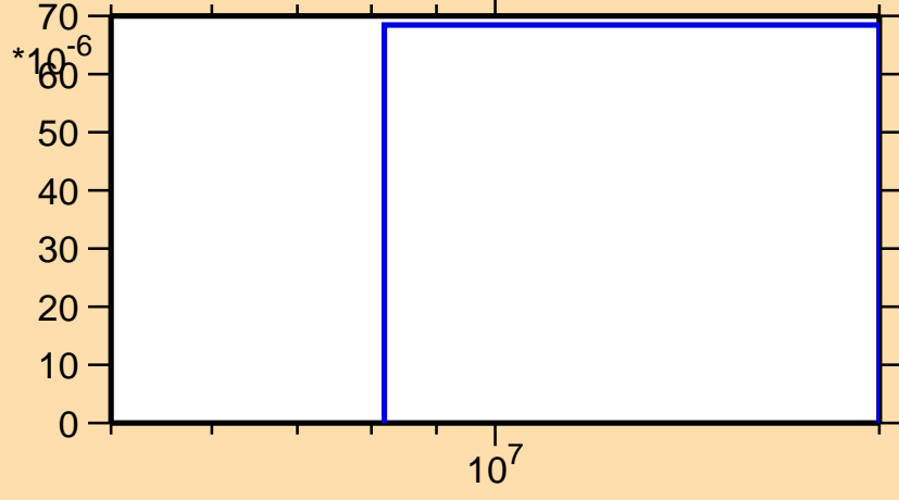
\sigma vs. E for ^{168}\text{Os}(n,t)
