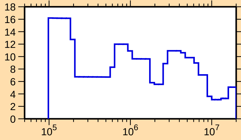
\Delta\sigma/\sigma vs. E for ^{169}\text{Os}(n,\text{tot.})
