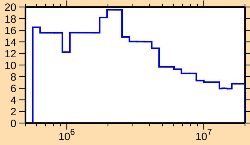
\Delta\sigma/\sigma vs. E for ^{169}\text{Os}(n,n\text{nonel.})
