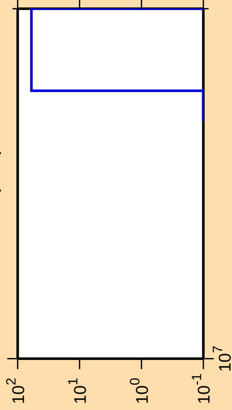
\Delta\sigma/\sigma vs. E for ^{169}\text{Os}(n,nt)
