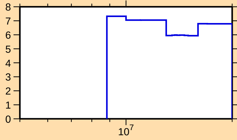
\Delta\sigma/\sigma vs. E for ^{169}\text{Os}(n,\text{nonel.})
