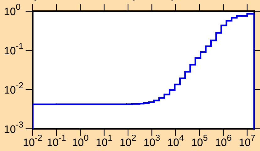
\mu vs. E for ^{169}\text{Os}(\text{mt251})
