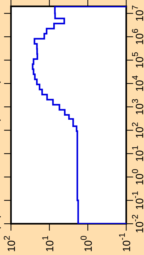
\Delta\mu/\mu vs. E for ^{169}\text{Os}(\text{mt251})
