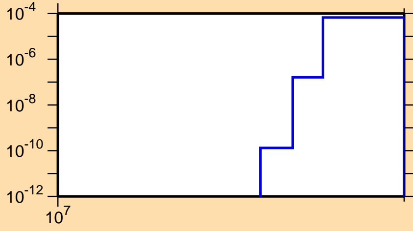
\sigma vs. E for ^{170}\text{Os}(n,2np)
