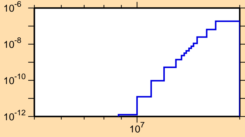
\sigma vs. E for ^{170}\text{Os}(\text{mt117})
