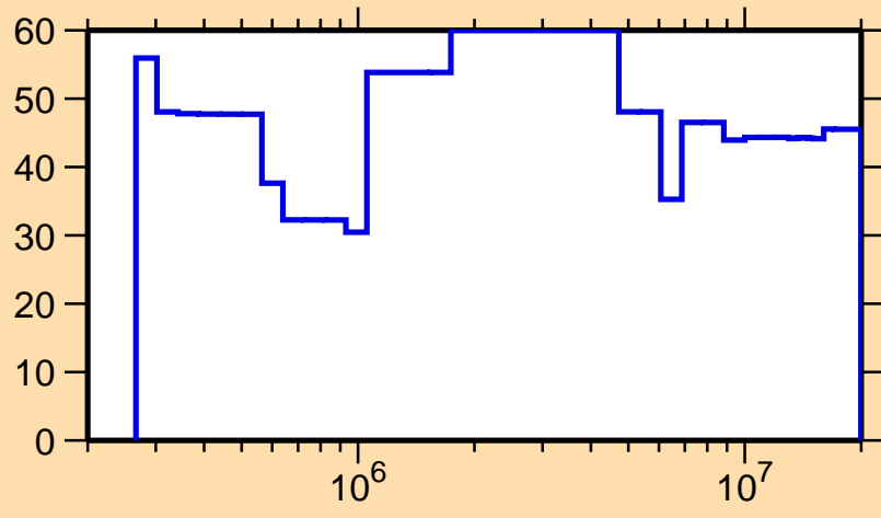
\Delta\sigma/\sigma vs. E for ^{170}\text{Os}(n,\text{inel.})
