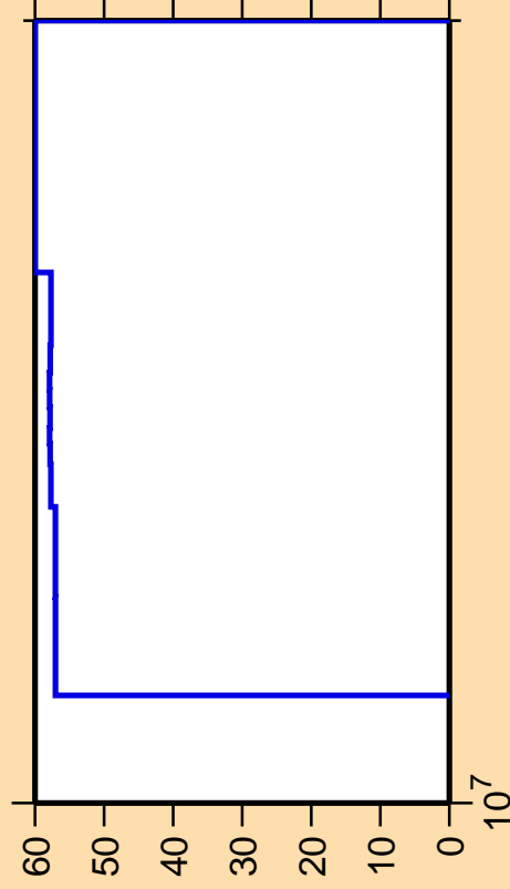
\Delta\sigma/\sigma vs. E for ^{170}\text{Os}(n,n\text{cont.})
