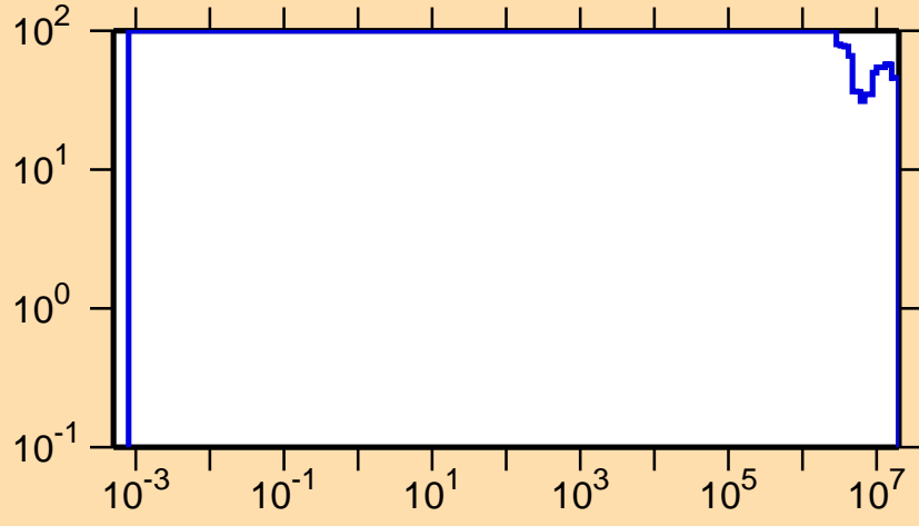
\Delta\sigma/\sigma vs. E for ^{170}\text{Os}(n,p)
