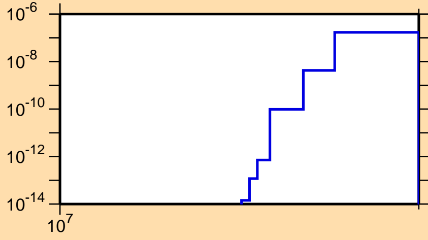
\sigma vs. E for ^{170}\text{Os}(n,\text{nd})
