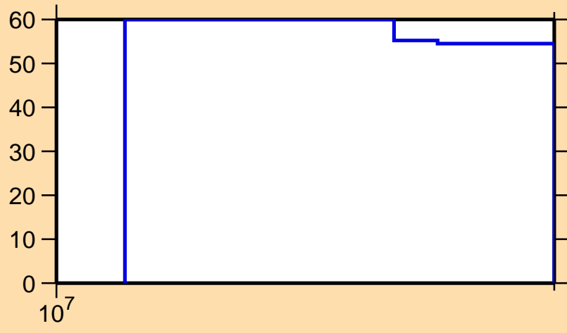
\Delta\sigma/\sigma vs. E for ^{170}\text{Os}(n,2n)
