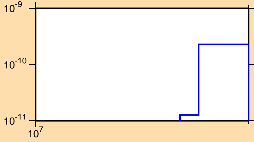
\sigma vs. E for ^{170}\text{Os} (mt 34)
