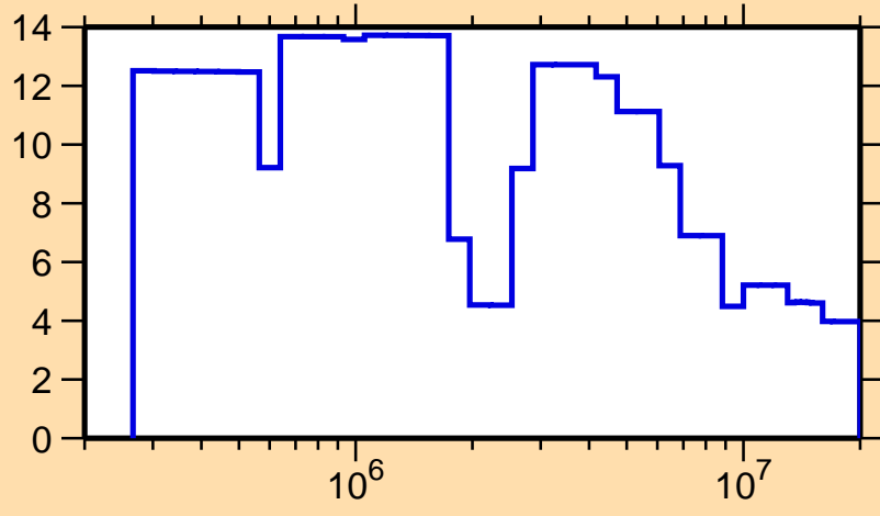
\Delta\sigma/\sigma vs. E for ^{170}\text{Os}(n,\text{tot.})
