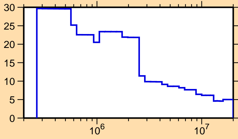
\Delta\sigma/\sigma vs. E for ^{170}\text{Os}(n,\text{nonel.})
