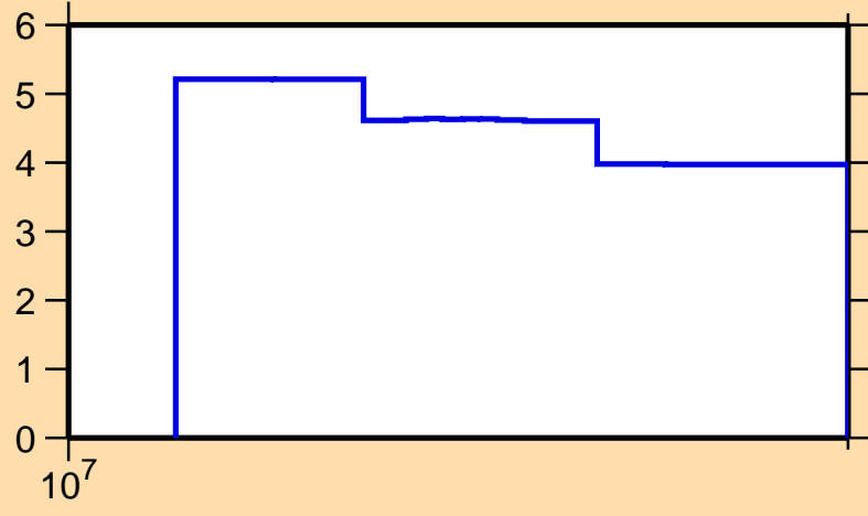
\Delta\sigma/\sigma vs. E for ^{170}\text{Os}(n,\text{tot.})
