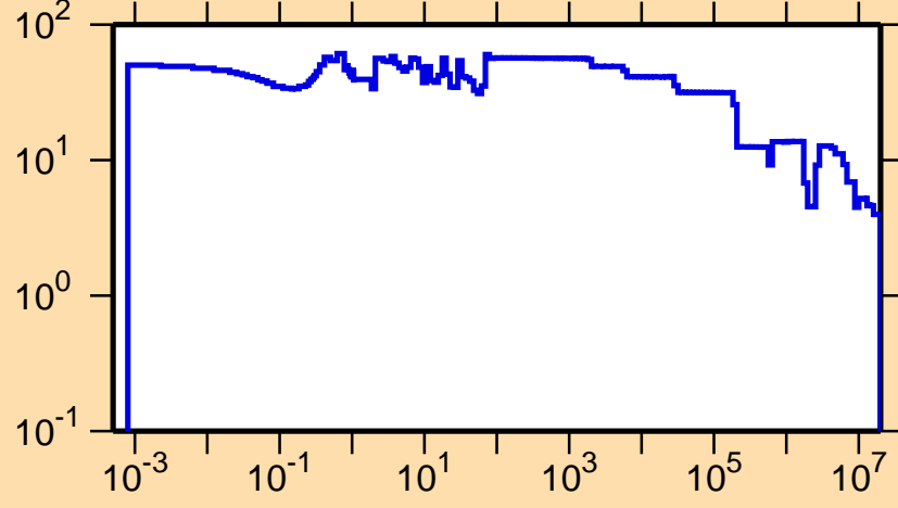
\Delta\sigma/\sigma vs. E for ^{170}\text{Os}(n,\text{tot.})
