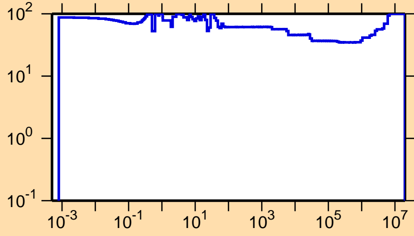
\Delta\sigma/\sigma vs. E for ^{170}\text{Os}(n,\gamma)
