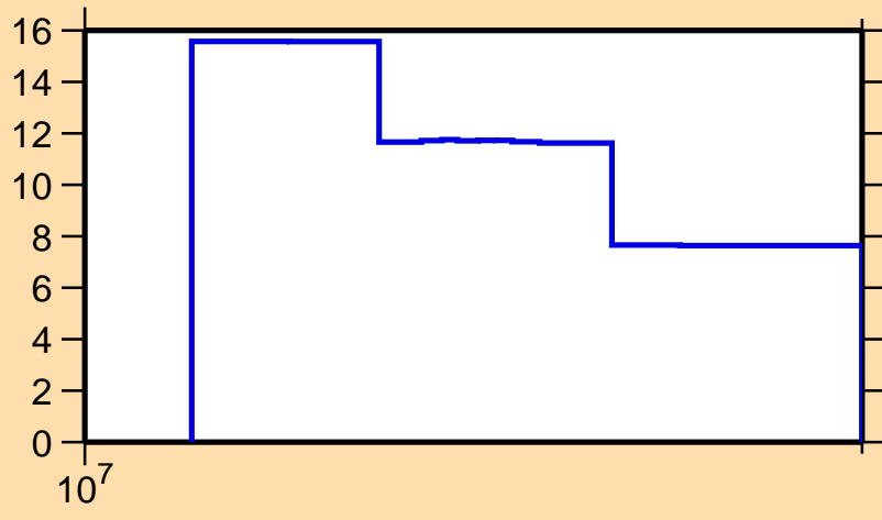
\Delta\sigma/\sigma vs. E for ^{170}\text{Os}(n,\text{el.})
