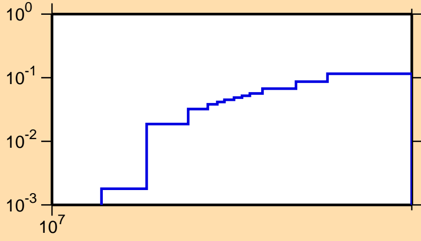
\sigma vs. E for ^{170}\text{Os}(n,2n)
