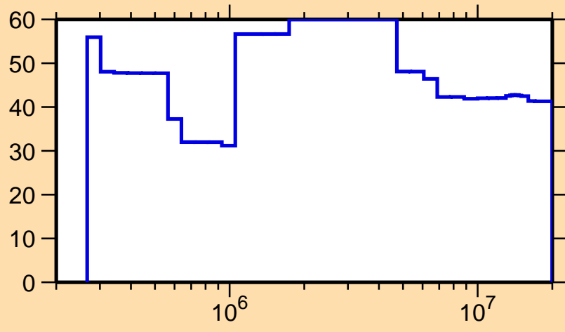
\Delta\sigma/\sigma vs. E for ^{170}\text{Os}(n,n_1)
