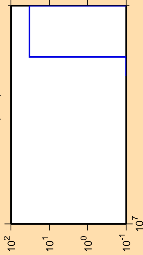
\Delta\sigma/\sigma vs. E for ^{170}\text{Os}(n,nt)
