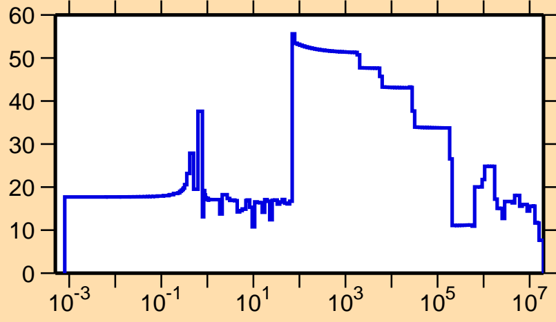
\Delta\sigma/\sigma vs. E for ^{170}\text{Os}(n,\text{el.})
