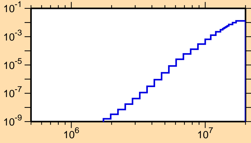
\sigma vs. E for ^{170}\text{Os}(n,p\alpha)
