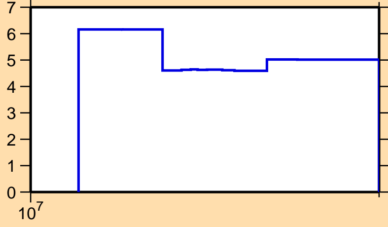
\Delta\sigma/\sigma vs. E for ^{170}\text{Os}(n,\text{nonel.})
