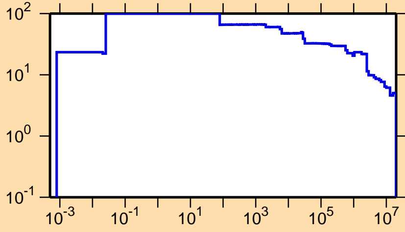
\Delta\sigma/\sigma vs. E for ^{170}\text{Os}(n,\text{nonel.})
