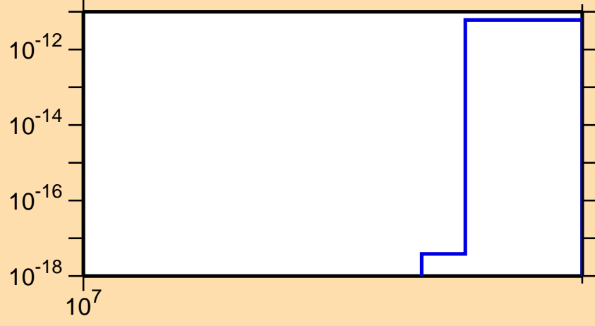
\sigma vs. E for ^{170}\text{Os}(n,nt)
