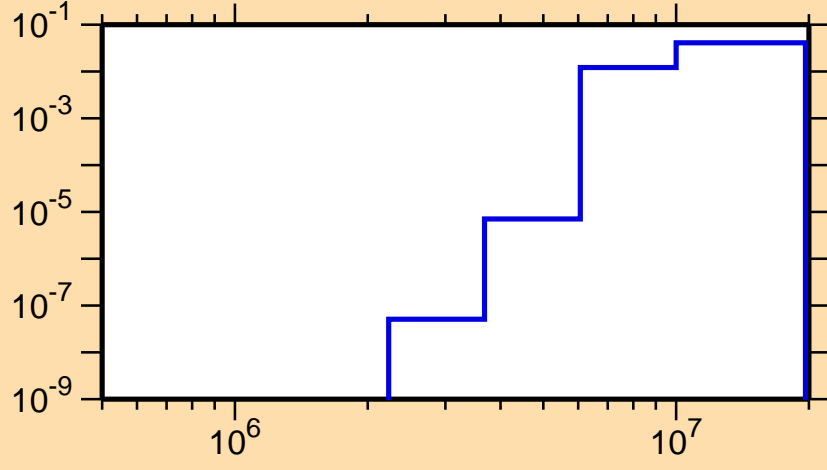
\sigma vs. E for ^{170}\text{Os}(n,n\alpha)
