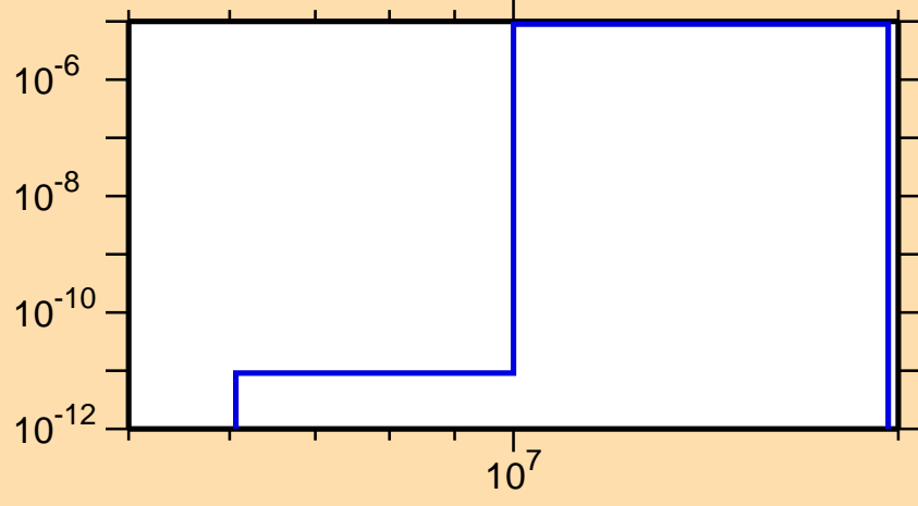
\sigma vs. E for ^{170}\text{Os}(n,pd)
