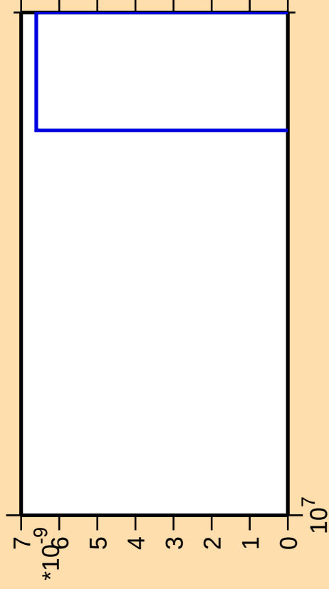
\Delta\sigma/\sigma vs. E for ^{171}\text{Os} (mt 11)
