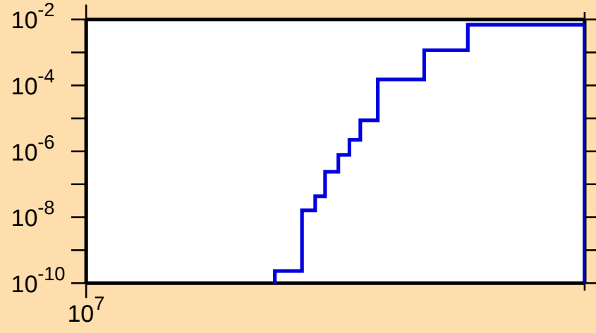
\sigma vs. E for ^{171}\text{Os}(n,2np)
