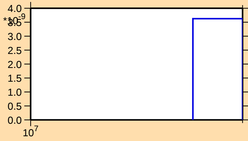
\sigma vs. E for ^{171}\text{Os}(n,3n)
