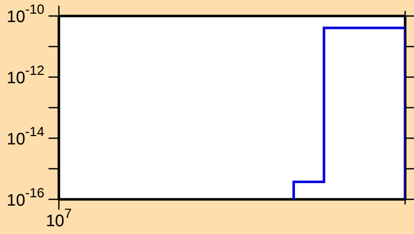
\sigma vs. E for ^{171}\text{Os}(n,nt)
