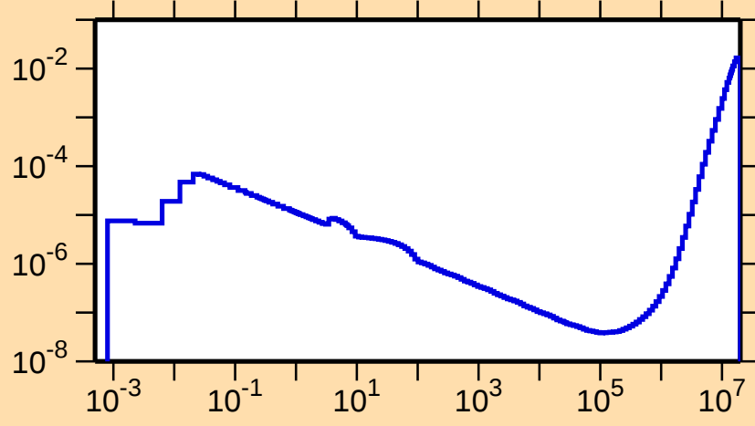
\sigma vs. E for ^{171}\text{Os}(n,p\alpha)
