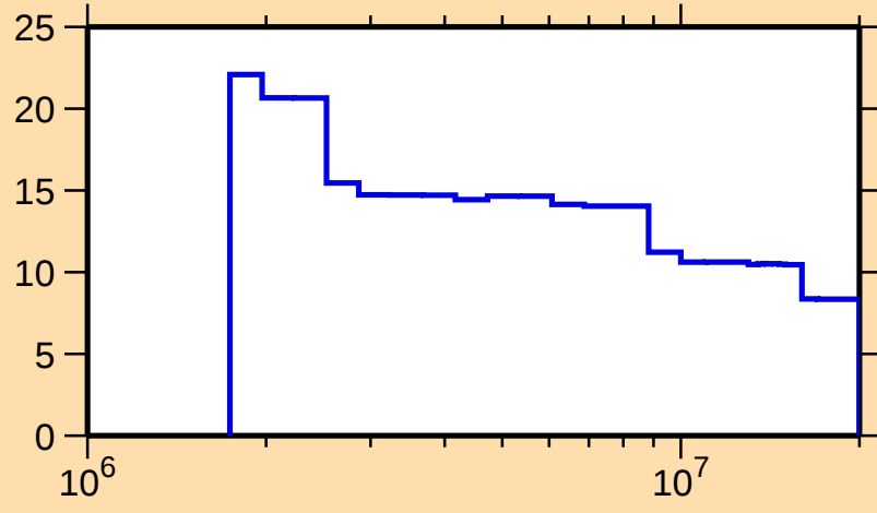
\Delta\sigma/\sigma vs. E for ^{171}\text{Os}(n,n\text{onel.})
