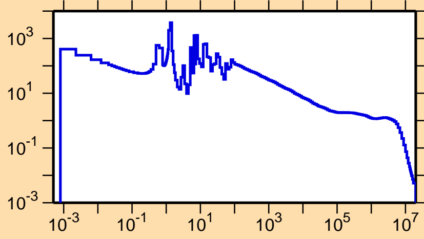
\sigma vs. E for ^{172}\text{Os}(n,\gamma)
