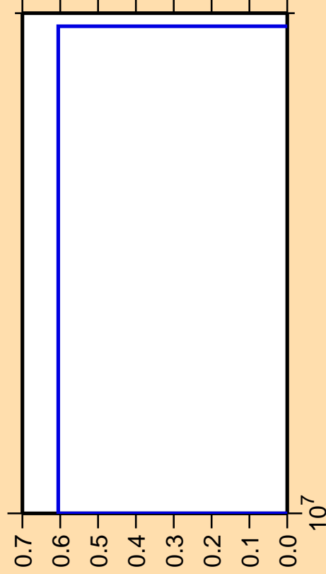
\Delta\sigma/\sigma vs. E for ^{172}\text{Os}(n,nt)
