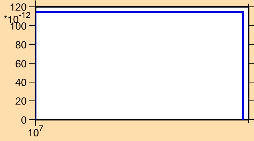
\sigma vs. E for ^{172}\text{Os}(n,\text{pt})
