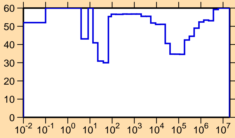
\Delta\sigma/\sigma vs. E for ^{172}\text{Os}(n,\gamma)
