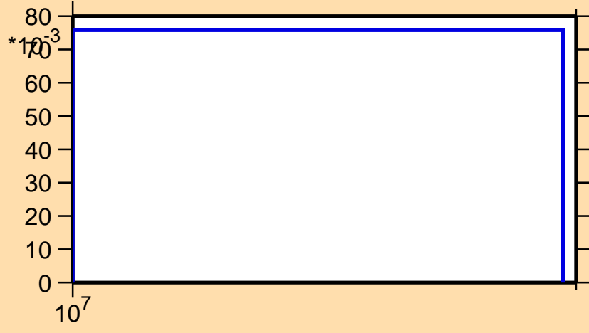
\sigma vs. E for ^{172}\text{Os}(n,2n)
