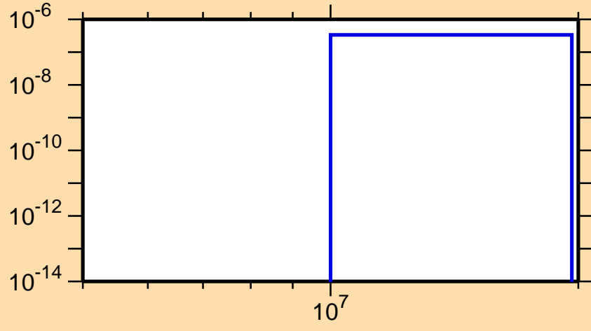
\sigma vs. E for ^{172}\text{Os}(n,2n\alpha)
