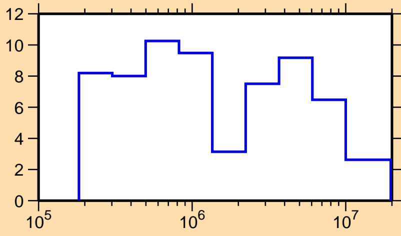
\Delta\sigma/\sigma vs. E for ^{172}\text{Os}(n,\text{tot.})
