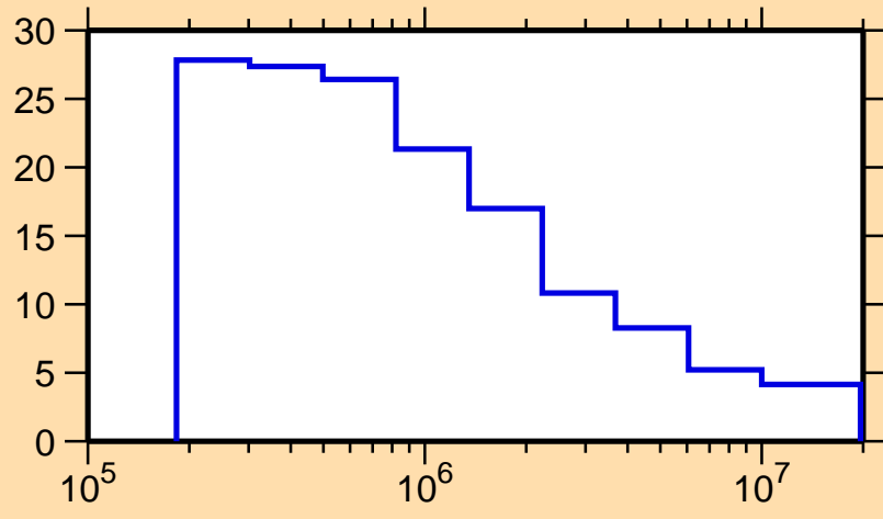
\Delta\sigma/\sigma vs. E for ^{172}\text{Os}(n,\text{nonel.})
