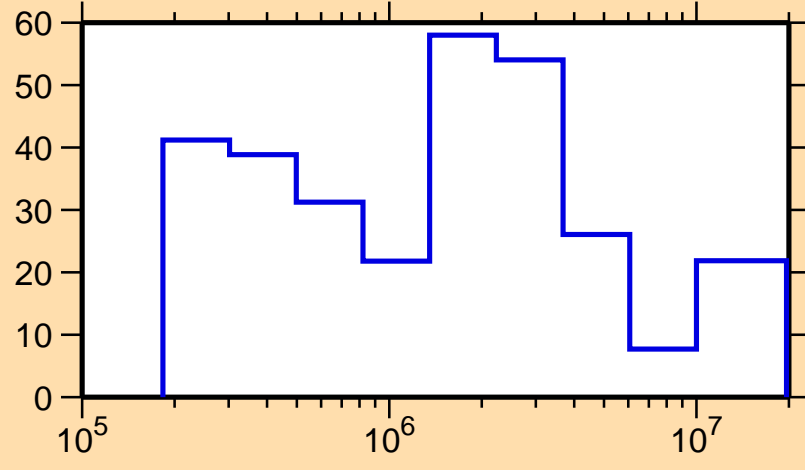
\Delta\sigma/\sigma vs. E for ^{172}\text{Os}(n,\text{inel.})
