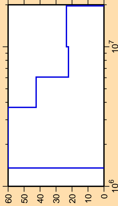
\Delta\sigma/\sigma vs. E for ^{172}\text{Os}(n,n_{\text{cont}}) .
