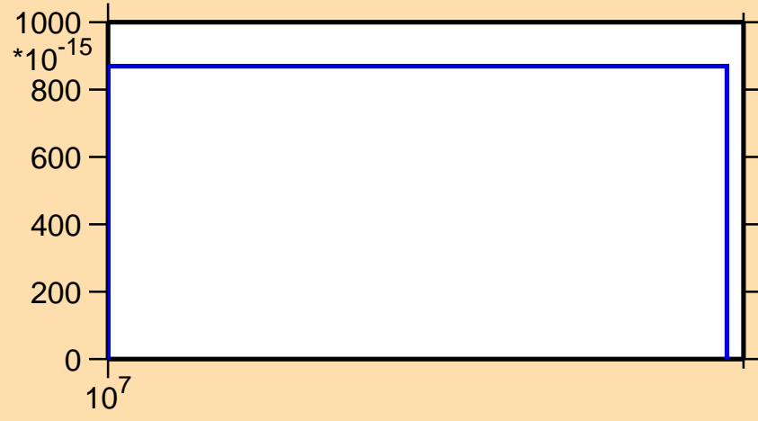
\sigma vs. E for ^{172}\text{Os} (mt 34)
