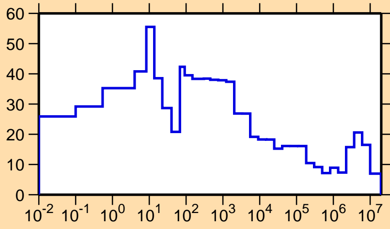
\Delta\sigma/\sigma vs. E for ^{172}\text{Os}(n,\text{el.})
