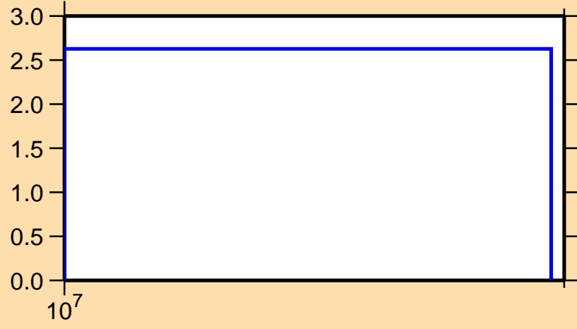
\Delta\sigma/\sigma vs. E for ^{172}\text{Os}(n,\text{tot.})
