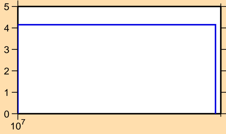
\Delta\sigma/\sigma vs. E for ^{172}\text{Os}(n,\text{nonel.})
