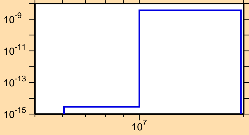
\sigma vs. E for ^{172}\text{Os}(\text{mt117})
