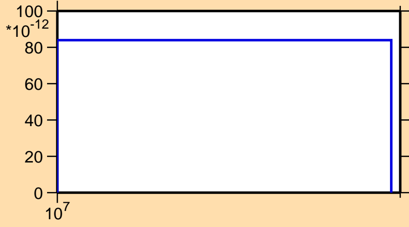
\sigma vs. E for ^{172}\text{Os}(n,3n)
