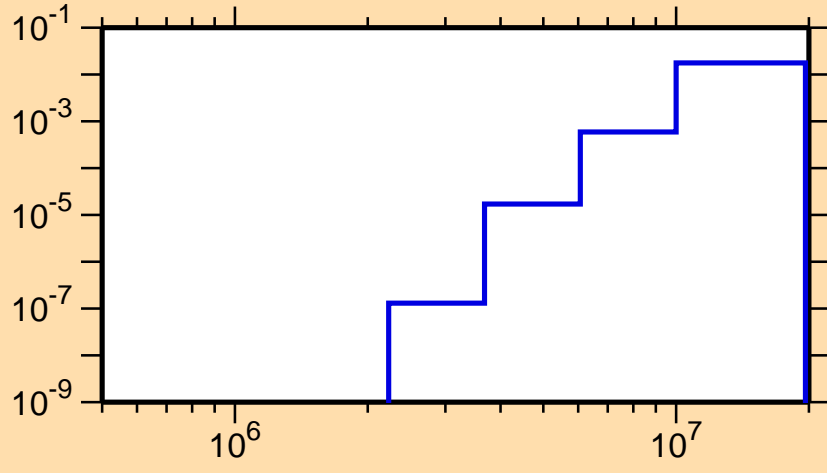
\sigma vs. E for ^{172}\text{Os}(n,n\alpha)
