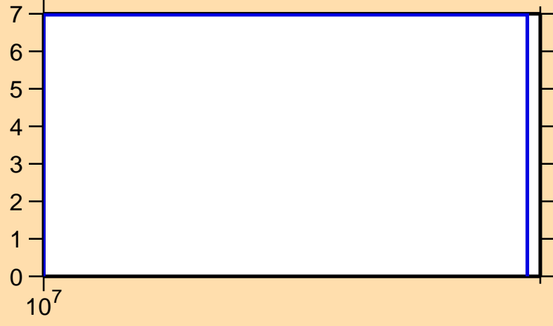
\Delta\sigma/\sigma vs. E for ^{172}\text{Os}(n,\text{el.})
