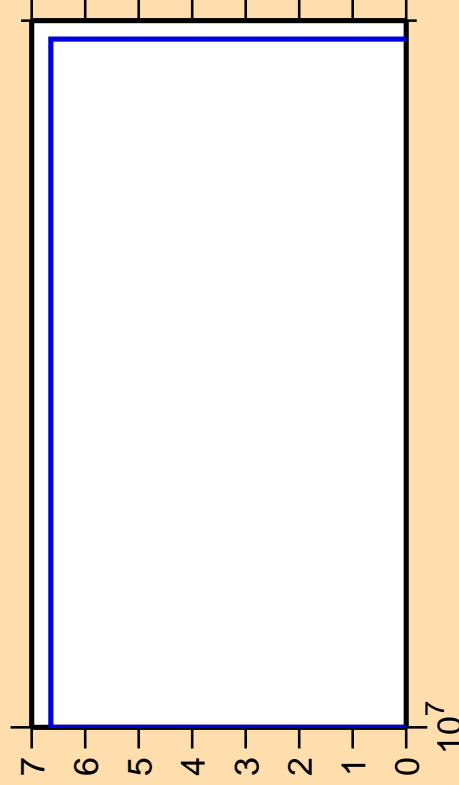
\Delta\sigma/\sigma vs. E for ^{172}\text{Os} (mt 34)
