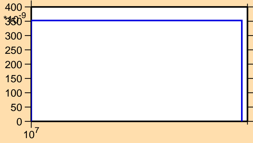
\sigma vs. E for ^{172}\text{Os}(n,2np)
