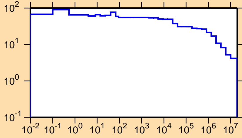
\Delta\sigma/\sigma vs. E for ^{172}\text{Os}(n,\text{nonel.})
