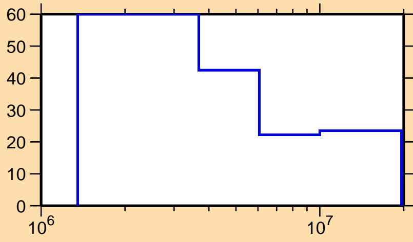
\Delta\sigma/\sigma vs. E for ^{172}\text{Os}(n,n\text{cont.})
