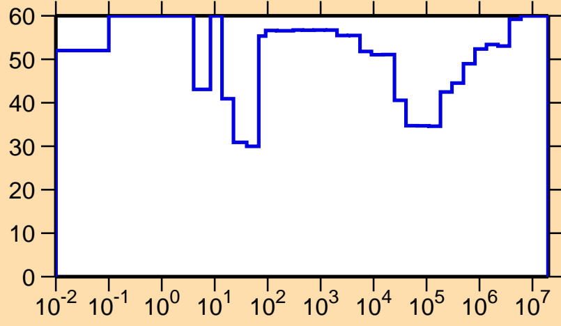
\Delta\sigma/\sigma vs. E for ^{172}\text{Os}(n,\gamma)
