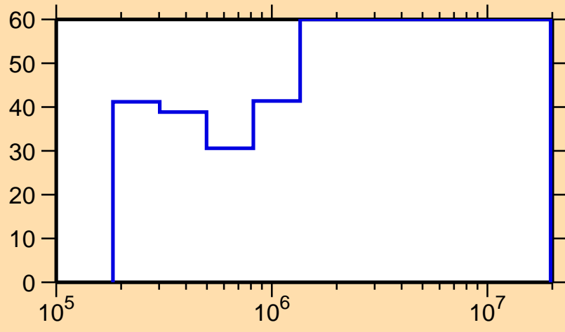
\Delta\sigma/\sigma vs. E for ^{172}\text{Os}(n,n_1)
