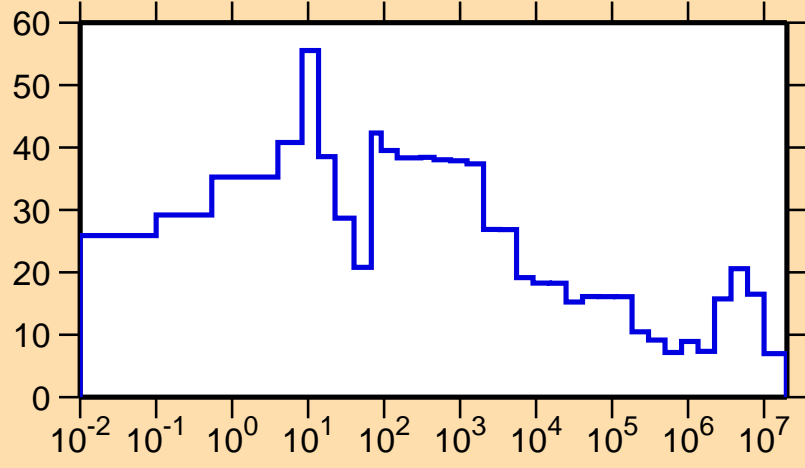
\Delta\sigma/\sigma vs. E for ^{172}\text{Os}(n,\text{el.})
