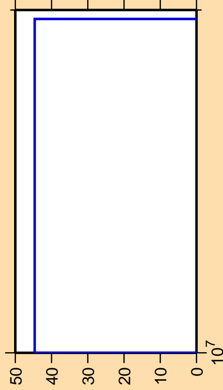
\Delta\sigma/\sigma vs. E for ^{172}\text{Os}(n,p)
