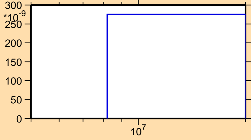
\sigma vs. E for ^{172}\text{Os}(n,2n\alpha)
