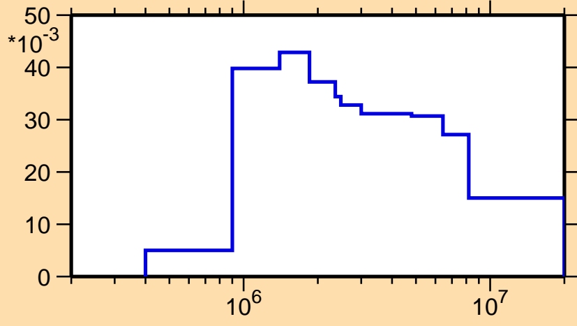
\sigma vs. E for ^{172}\text{Os}(n,n_2)
