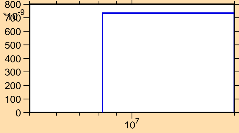
\sigma vs. E for ^{172}\text{Os}(n,\text{pd})
