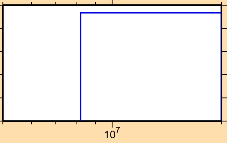
\sigma vs. E for ^{172}\text{Os}(n,t)
