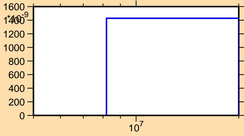
\sigma vs. E for ^{172}\text{Os} (mt 45)
