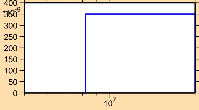
\sigma vs. E for ^{172}\text{Os}(n,2np)
