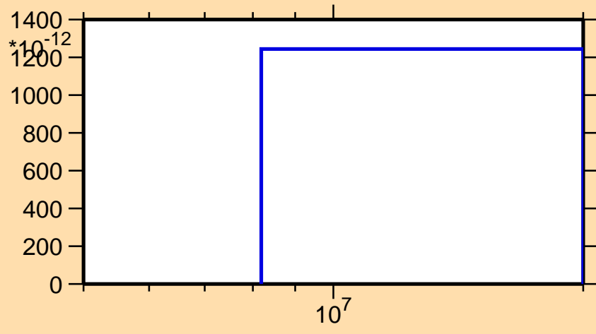
\sigma vs. E for ^{172}\text{Os}(n,\text{nd})
