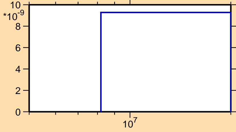
\sigma vs. E for ^{173}\text{Os}(n,3n)
