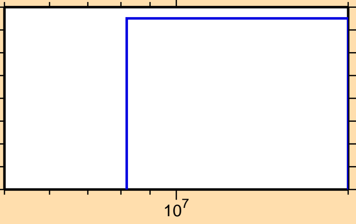
\sigma vs. E for ^{173}\text{Os}(n,\text{nd})
