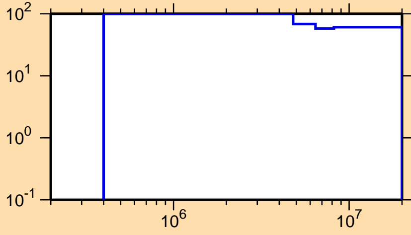
\Delta\sigma/\sigma vs. E for ^{173}\text{Os}(n,n\text{cont.})
