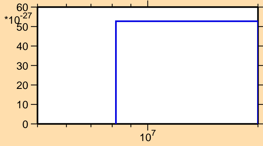
\sigma vs. E for ^{173}\text{Os} (mt 11)
