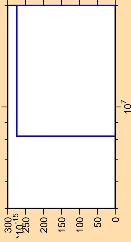
\Delta\sigma/\sigma vs. E for ^{173}\text{Os} (mt 11)
