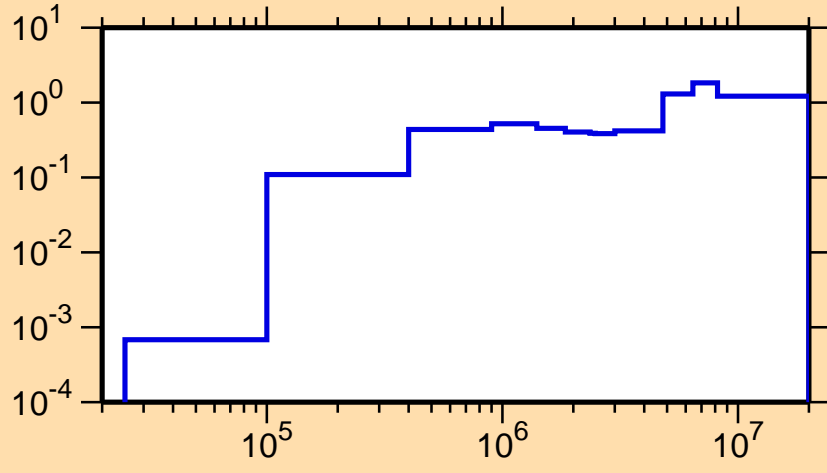
\sigma vs. E for ^{173}\text{Os}(n,\text{inel.})
