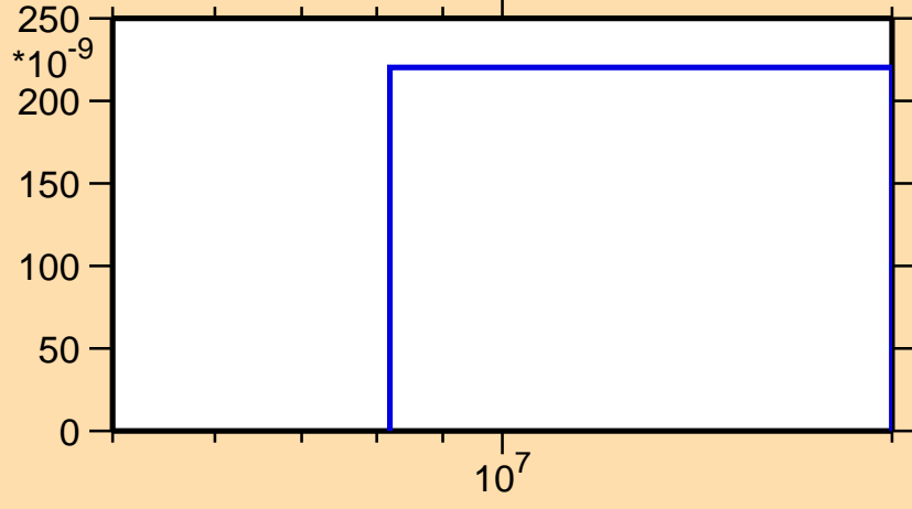
\sigma vs. E for ^{173}\text{Os}(n,\text{pd})
