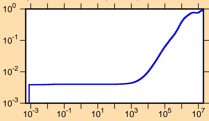
\mu vs. E for ^{174}\text{Os}(\text{mt251})
