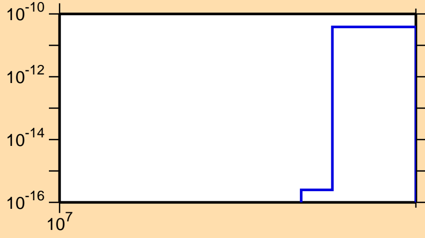
\sigma vs. E for ^{174}\text{Os}(n,nt)
