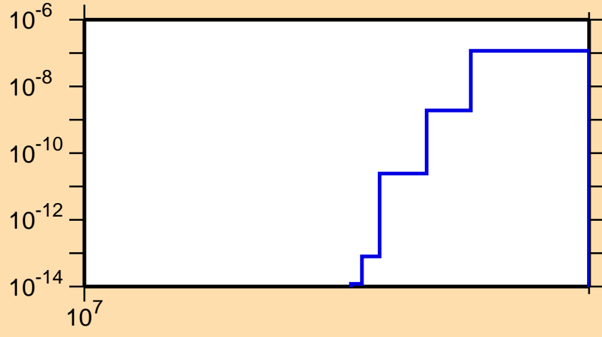
\sigma vs. E for ^{174}\text{Os}(n,\text{nd})
