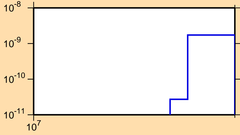
\sigma vs. E for ^{174}\text{Os}(n,\text{pt})
