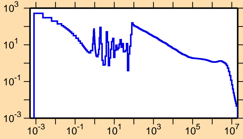
\sigma vs. E for ^{174}\text{Os}(n,\gamma)
