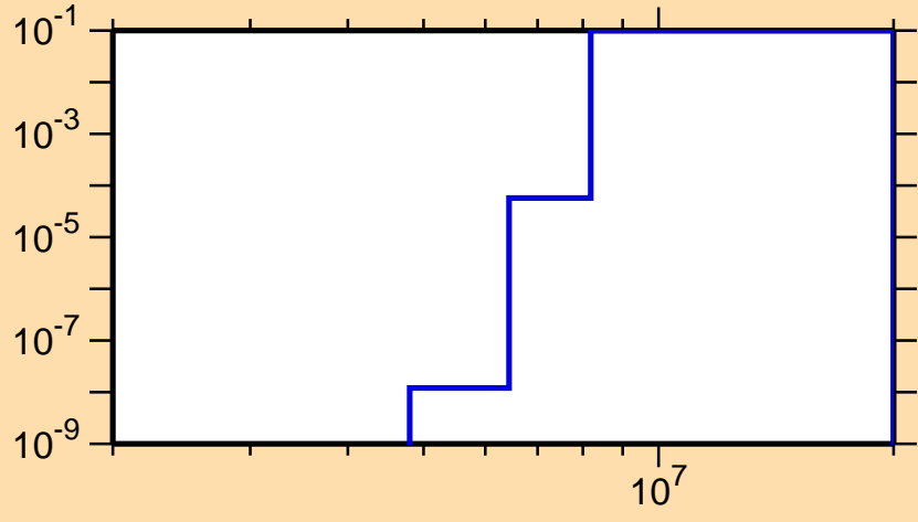
\sigma vs. E for ^{174}\text{Os}(n,np)
