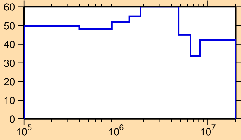
\Delta\sigma/\sigma vs. E for ^{174}\text{Os}(n,\text{inel.})
