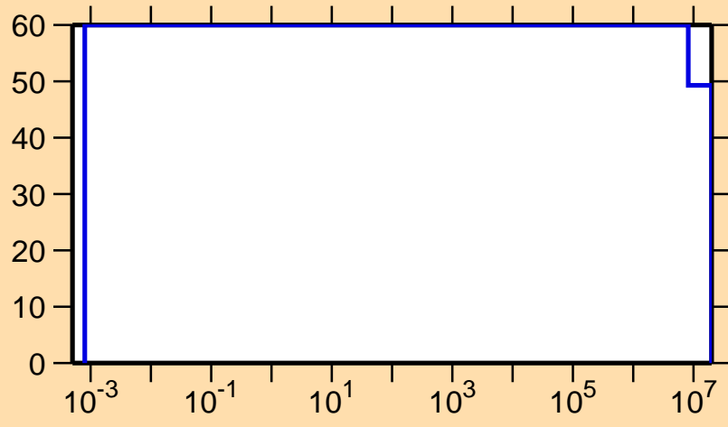
\Delta\sigma/\sigma vs. E for ^{174}\text{Os}(n,p)
