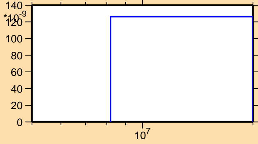
\sigma vs. E for ^{174}\text{Os} (mt 45)
