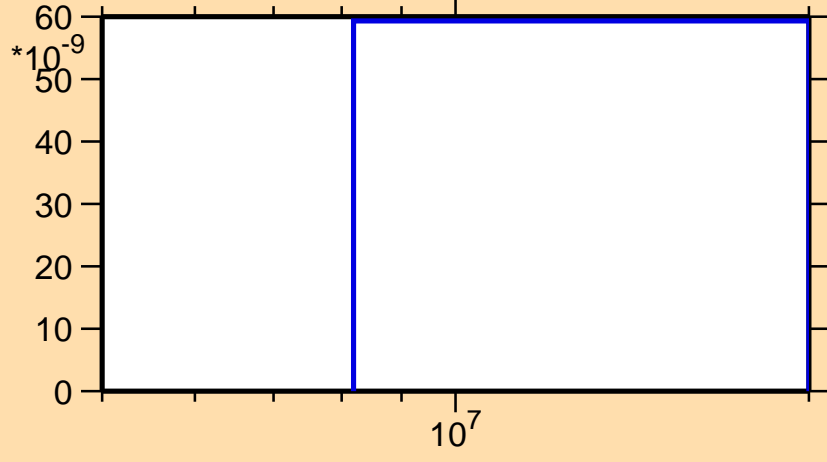
\sigma vs. E for ^{174}\text{Os}(n,\text{pd})
