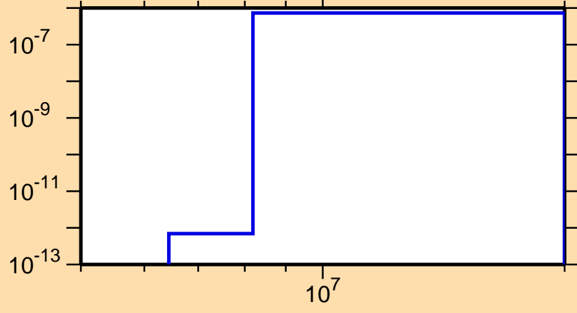
\sigma vs. E for ^{174}\text{Os}(n,\text{He}3)
