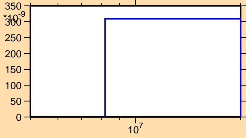
\sigma vs. E for ^{174}\text{Os}(n,2n\alpha)
