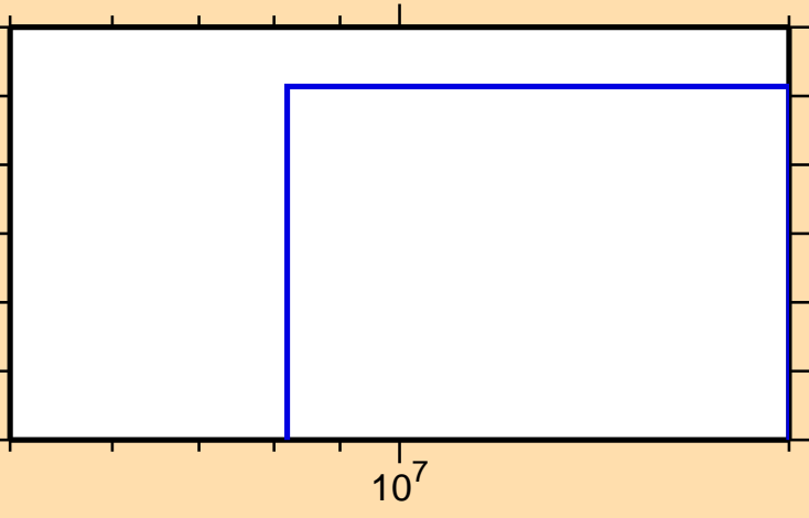
\sigma vs. E for ^{174}\text{Os}(n,\text{nd})
