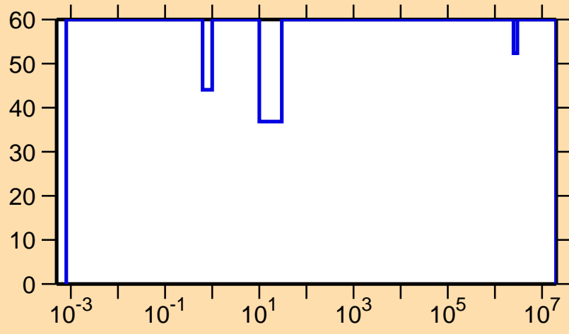
\Delta\sigma/\sigma vs. E for ^{174}\text{Os}(n,\gamma)
