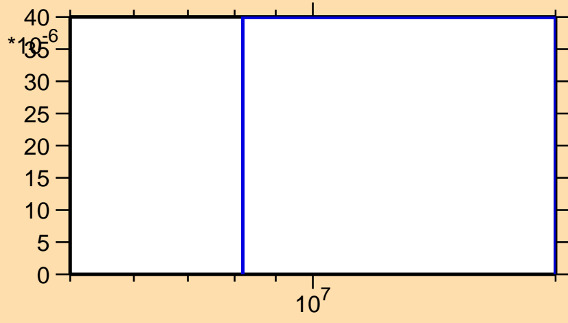
\sigma vs. E for ^{174}\text{Os}(n,t)
