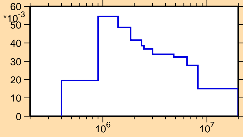
\sigma vs. E for ^{174}\text{Os}(n,n_2)
