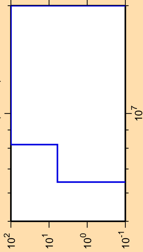
\Delta\sigma/\sigma vs. E for ^{174}\text{Os}(n,\text{He}3)
