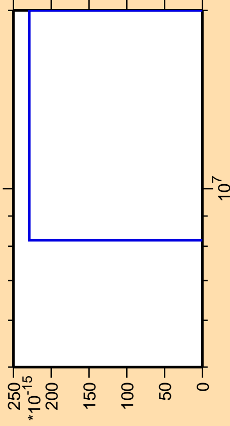
\Delta\sigma/\sigma vs. E for ^{175}\text{Os} (mt 11)
