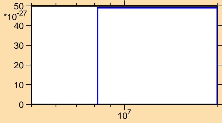
\sigma vs. E for ^{175}\text{Os} (mt 11)
