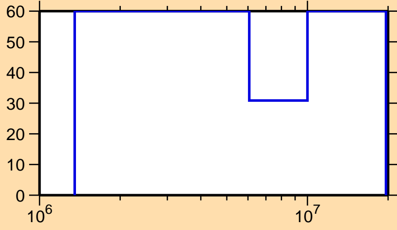
\Delta\sigma/\sigma vs. E for ^{176}\text{Os}(n,n\text{cont.})
