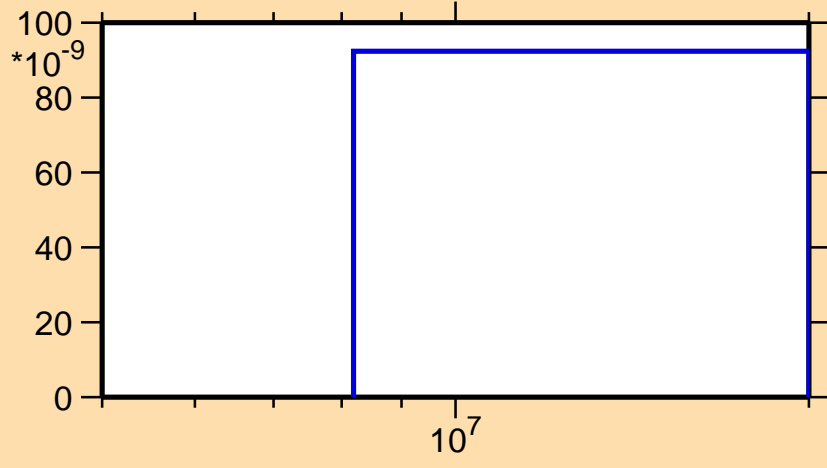
\sigma vs. E for ^{176}\text{Os}(n,2np)
