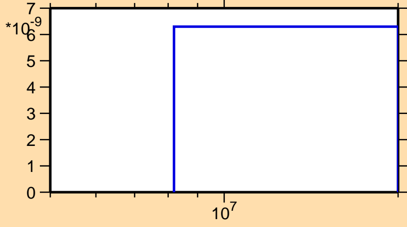
\sigma vs. E for ^{176}\text{Os} (mt 45)
