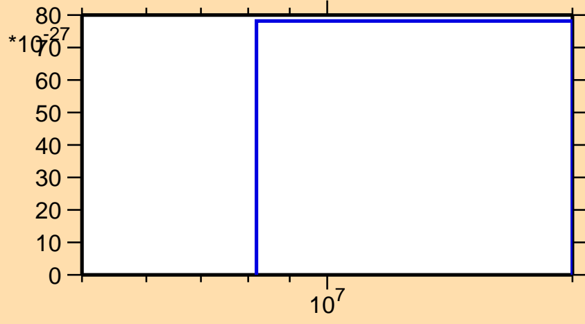
\sigma vs. E for ^{176}\text{Os} (mt 11)
