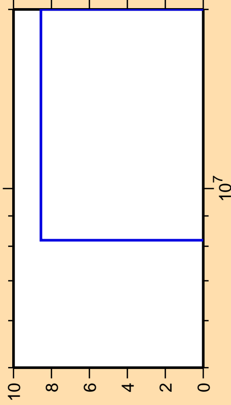
\Delta\sigma/\sigma vs. E for ^{176}\text{Os}(n,nt)
