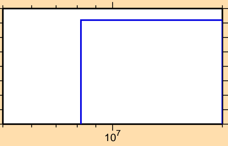
\sigma vs. E for ^{176}\text{Os}(n,t)
