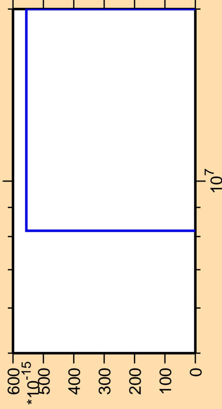
\Delta\sigma/\sigma vs. E for ^{176}\text{Os} (mt 11)
