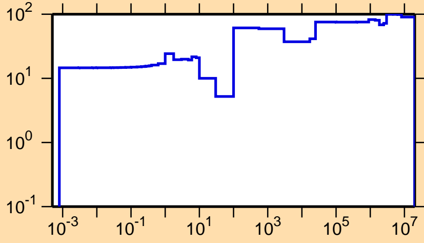
\Delta\sigma/\sigma vs. E for ^{176}\text{Os}(n,\gamma)
