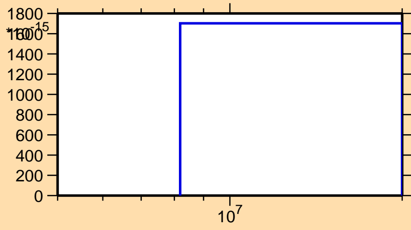
\sigma vs. E for ^{176}\text{Os}(n,\text{pt})
