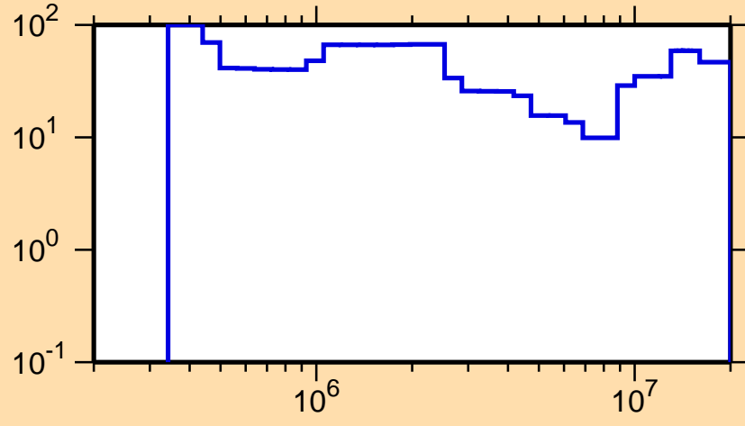
\Delta\sigma/\sigma vs. E for ^{177}\text{Os}(n,n\text{cont.})
