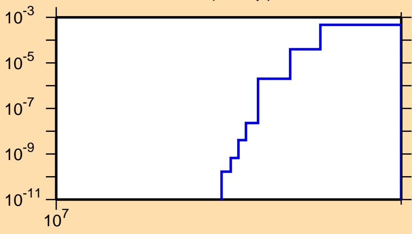
\sigma vs. E for ^{177}\text{Os}(n,2np)
