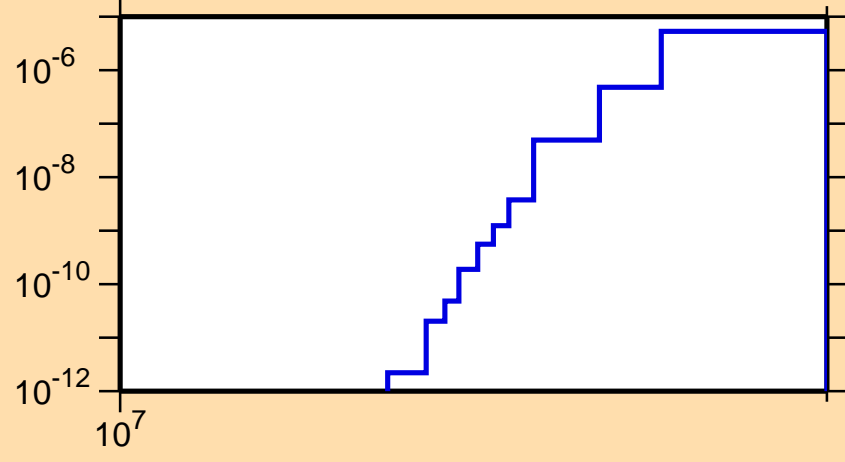
\sigma vs. E for ^{177}\text{Os}(n,\text{nd})
