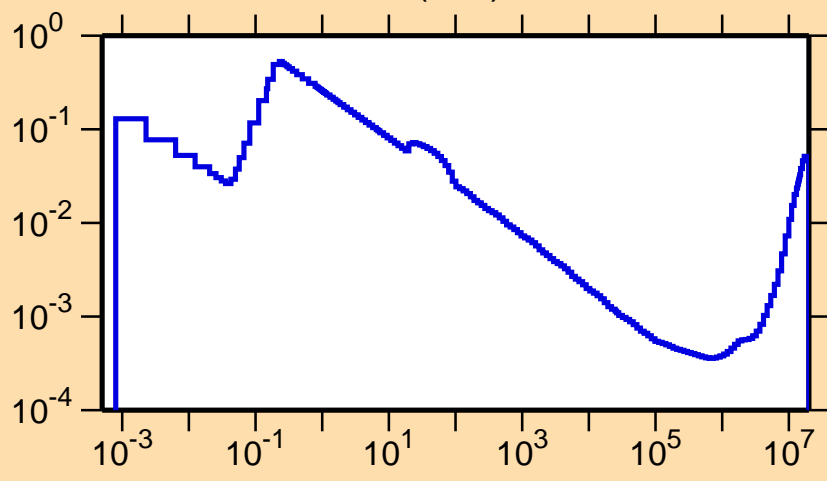
\sigma vs. E for ^{177}\text{Os}(n,\alpha)
