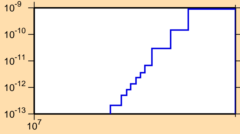
\sigma vs. E for ^{177}\text{Os}(\text{mt117})
