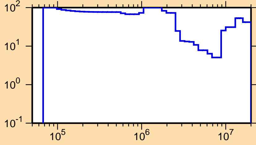
\Delta\sigma/\sigma vs. E for ^{177}\text{Os}(n,\text{inel.})
