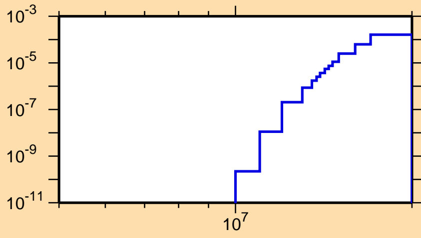
\sigma vs. E for ^{177}\text{Os}(n,2n\alpha)
