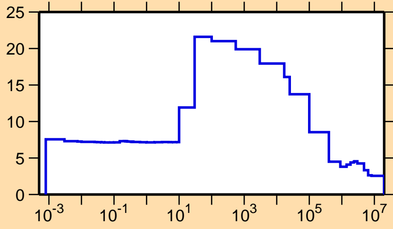
\sigma vs. E for ^{177}\text{Os}(n,\text{el.})
