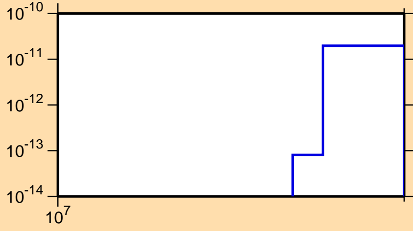
\sigma vs. E for ^{178}\text{Os}(n,\text{pt})
