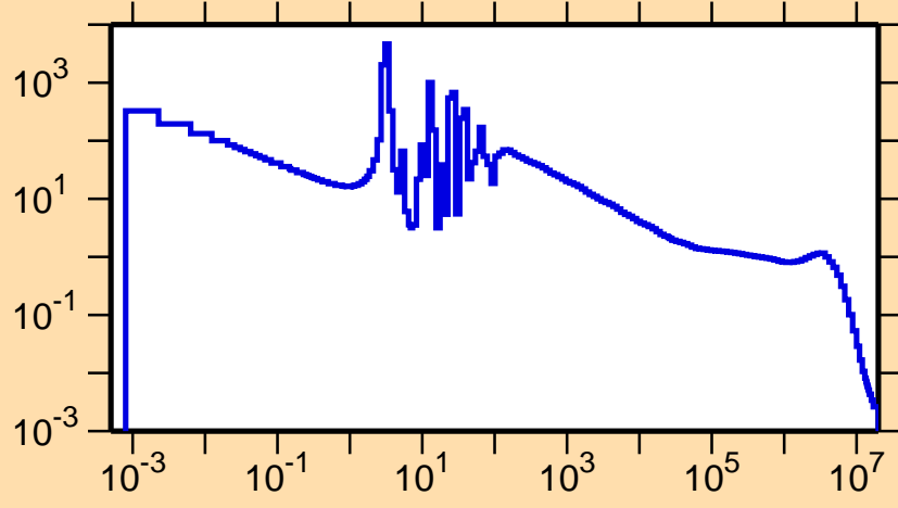
\sigma vs. E for ^{178}\text{Os}(n,\gamma)
