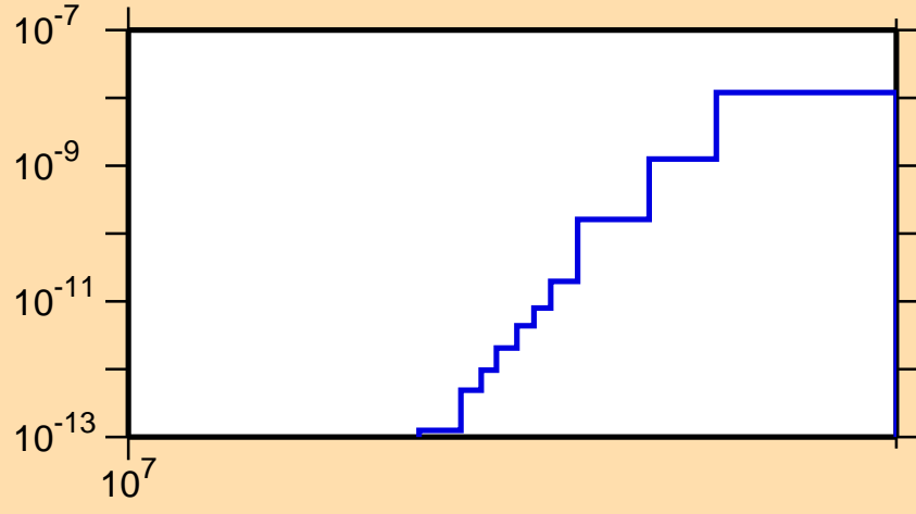
\sigma vs. E for ^{178}\text{Os}(n,\text{pd})
