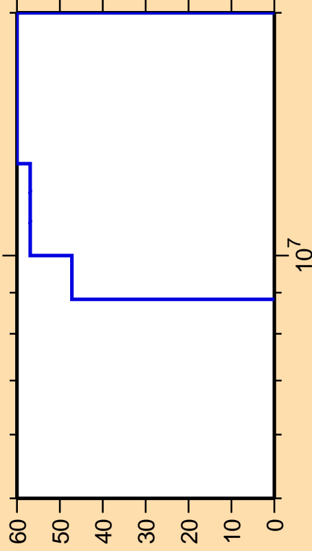
\Delta\sigma/\sigma vs. E for ^{178}\text{Os}(n,n\text{cont.})
