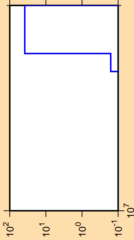
\Delta\sigma/\sigma vs. E for ^{178}\text{Os} (mt 34)
