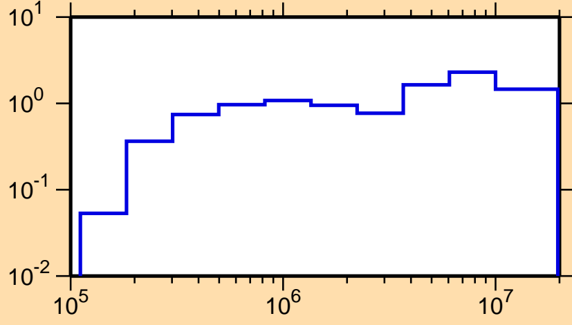
\sigma vs. E for ^{178}\text{Os}(n,\text{inel.})
