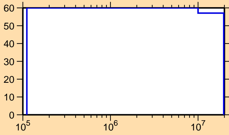
\Delta\sigma/\sigma vs. E for ^{178}\text{Os}(n,n_1)
