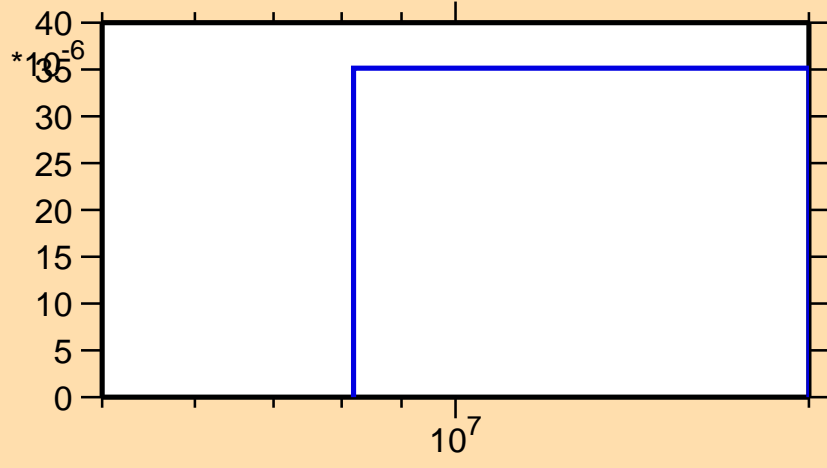
\sigma vs. E for ^{178}\text{Os}(n,t)
