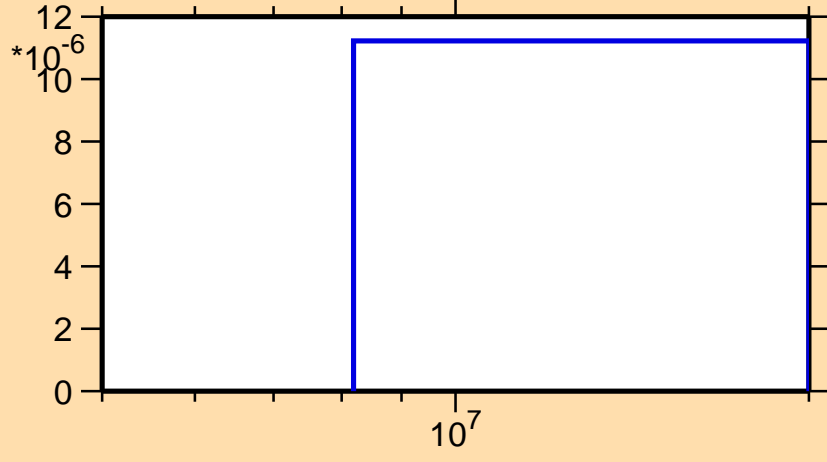
\sigma vs. E for ^{178}\text{Os}(n,3n)
