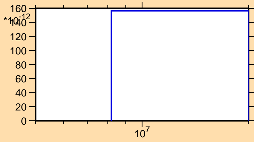
\sigma vs. E for ^{178}\text{Os} (mt 45)
