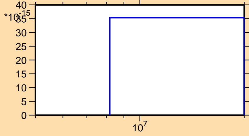
\sigma vs. E for ^{178}\text{Os} (mt 34)
