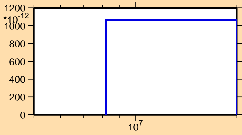
\sigma vs. E for ^{178}\text{Os}(n,\text{nd})
