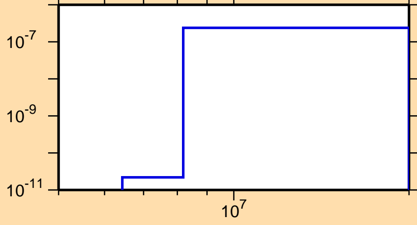
\sigma vs. E for ^{178}\text{Os}(n,p\alpha)
