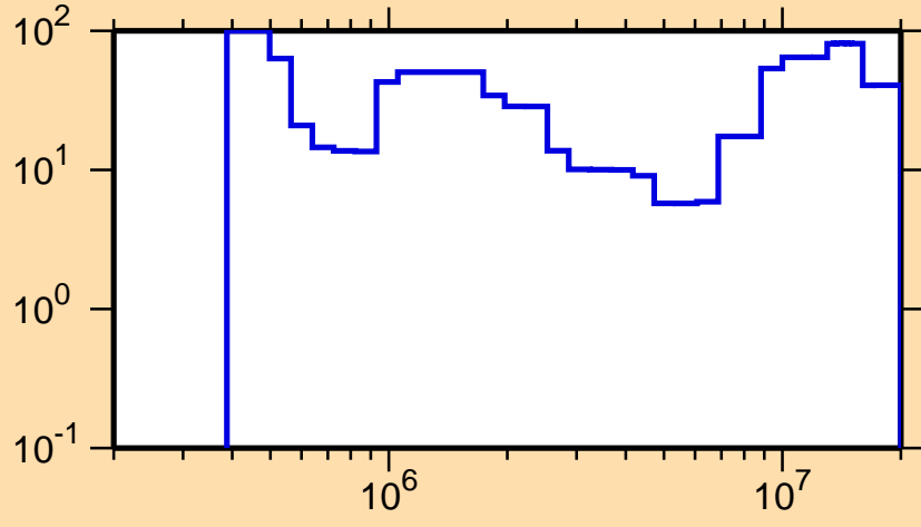
\Delta\sigma/\sigma vs. E for ^{179}\text{Os}(n,n\text{cont.})
