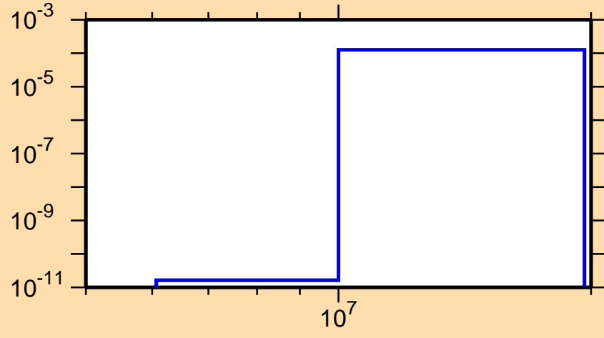
\sigma vs. E for ^{179}\text{Os}(n,t)
