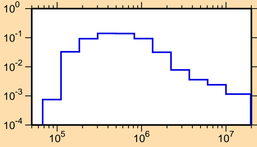
\sigma vs. E for ^{179}\text{Os}(n,n_2)
