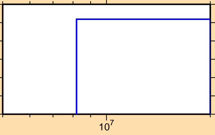
\sigma vs. E for ^{179}\text{Os}(n,nt)
