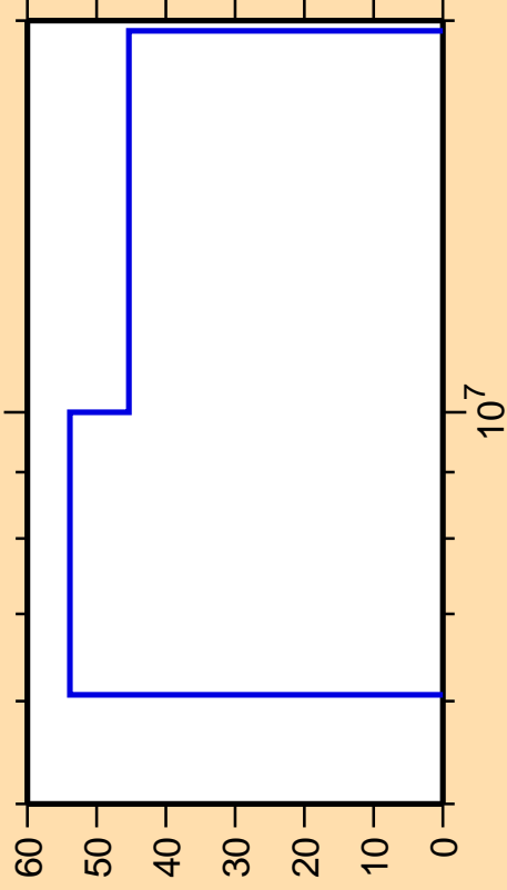
\Delta\sigma/\sigma vs. E for ^{180}\text{Os}(n,np)
