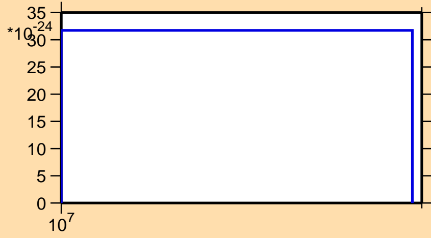
\sigma vs. E for ^{180}\text{Os} (mt 11)
