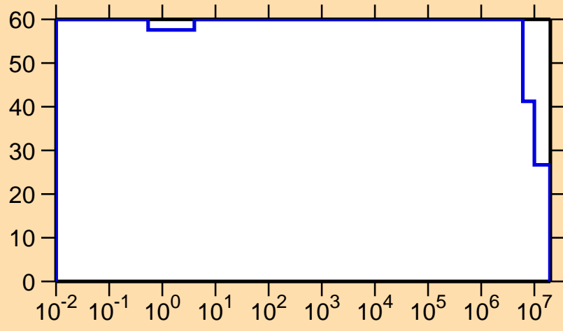
\Delta\sigma/\sigma vs. E for ^{180}\text{Os}(n,p)
