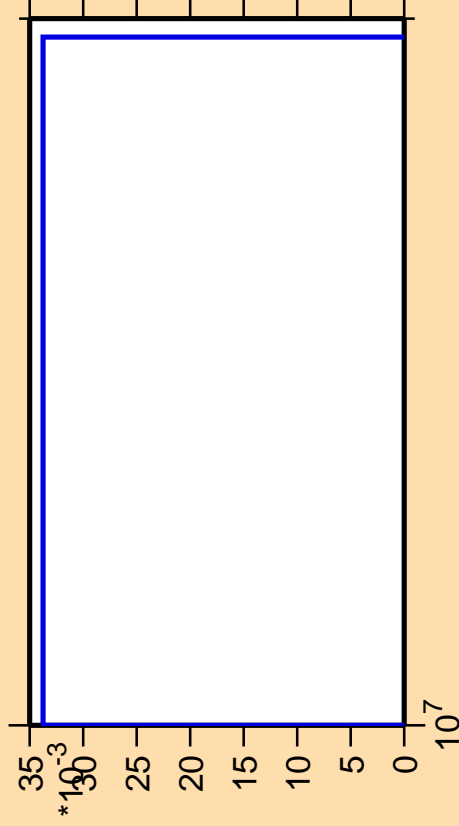
\Delta\sigma/\sigma vs. E for ^{180}\text{Os} (mt 34)
