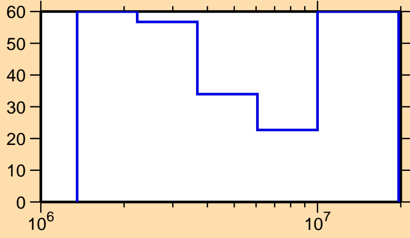
\Delta\sigma/\sigma vs. E for ^{180}\text{Os}(n,n\text{cont.})
