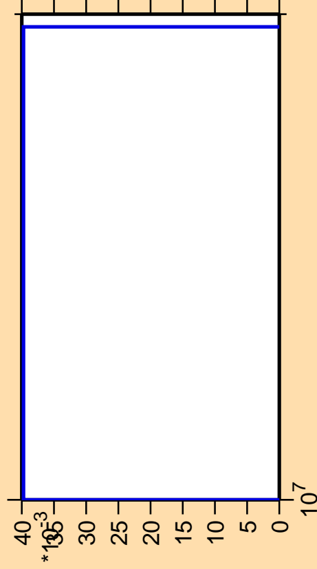
\Delta\sigma/\sigma vs. E for ^{180}\text{Os}(n,\text{pt})
