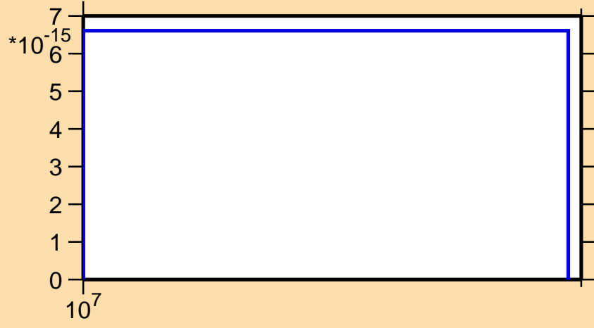
\sigma vs. E for ^{180}\text{Os}(n,\text{pt})
