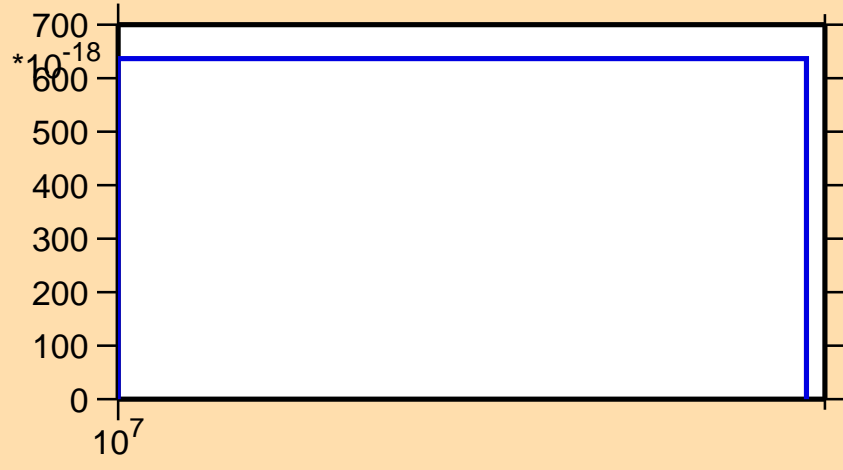
\sigma vs. E for ^{180}\text{Os}(n,3n\alpha)
