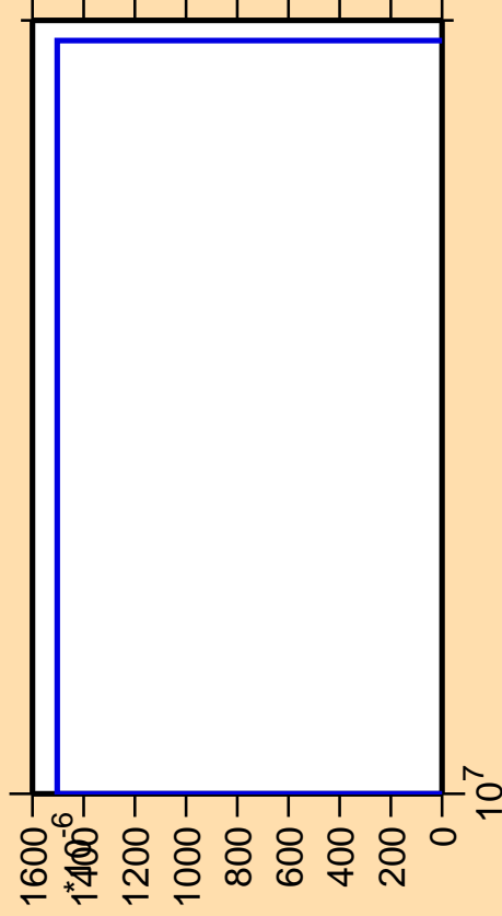
\Delta\sigma/\sigma vs. E for ^{180}\text{Os}(n,3n\alpha)
