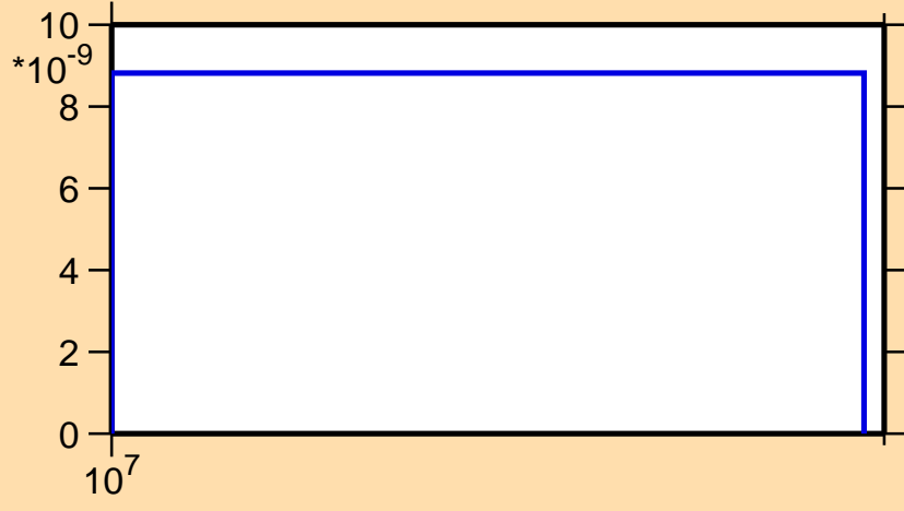
\sigma vs. E for ^{180}\text{Os}(n,2np)
