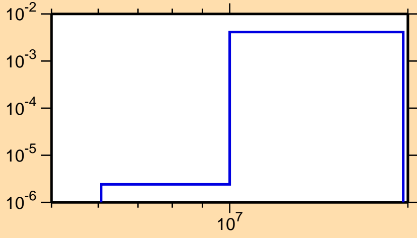
\sigma vs. E for ^{180}\text{Os}(n,np)
