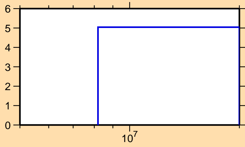
\Delta\sigma/\sigma vs. E for ^{180}\text{Os}(n,\text{tot.})
