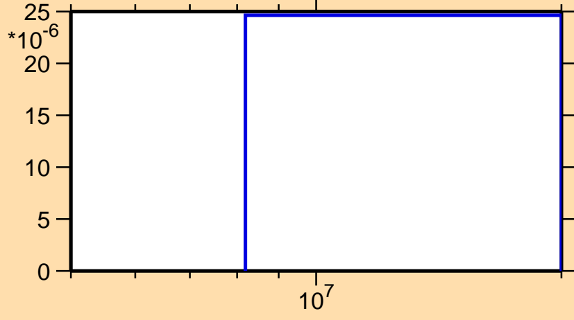
\sigma vs. E for ^{180}\text{Os}(n,t)
