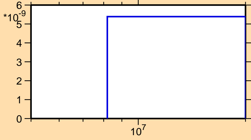
\sigma vs. E for ^{180}\text{Os}(n,\text{He}3)
