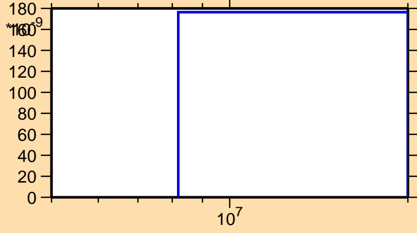
\sigma vs. E for ^{180}\text{Os}(n,2n\alpha)
