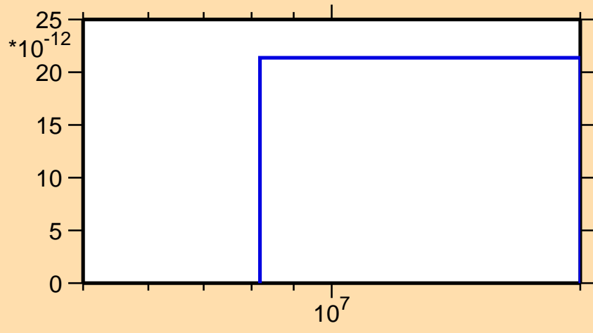
\sigma vs. E for ^{180}\text{Os} (mt 45)
