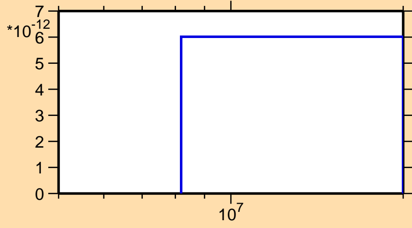
\sigma vs. E for ^{180}\text{Os}(n,pd)
