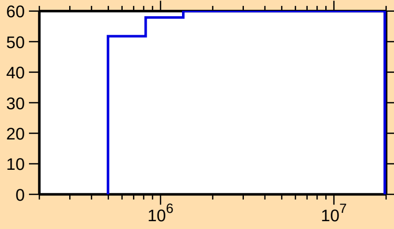
\Delta\sigma/\sigma vs. E for ^{181}\text{Os}(n,n_1)
