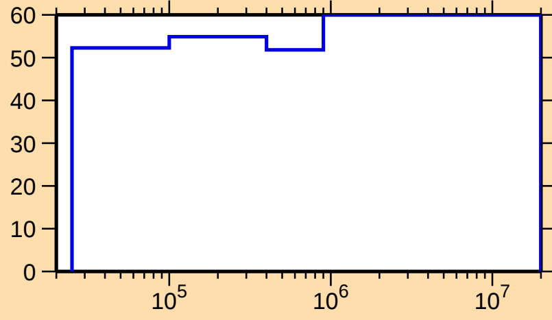
\Delta\sigma/\sigma vs. E for ^{181}\text{Os}(n,n_1)
