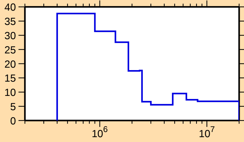
\Delta\sigma/\sigma vs. E for ^{181}\text{Os}(n,n\text{onel.})
