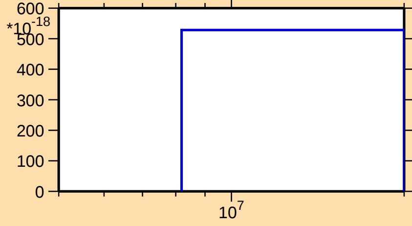
\sigma vs. E for ^{181}\text{Os}(n,3n\alpha)
