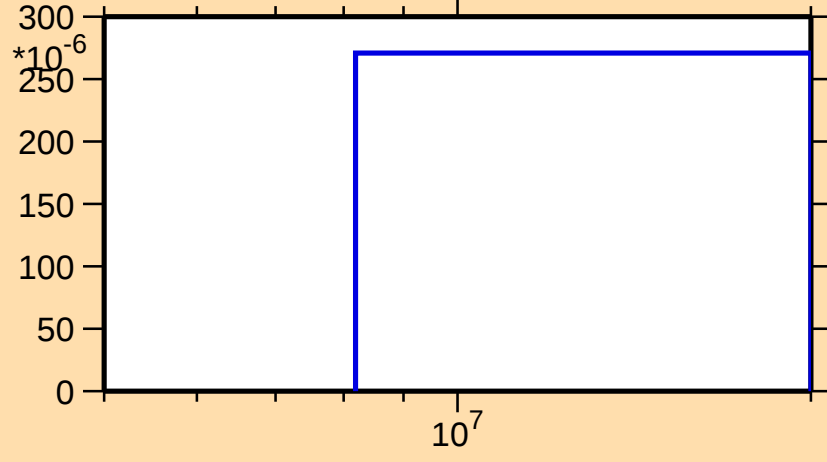
\sigma vs. E for ^{181}\text{Os}(n,3n)
