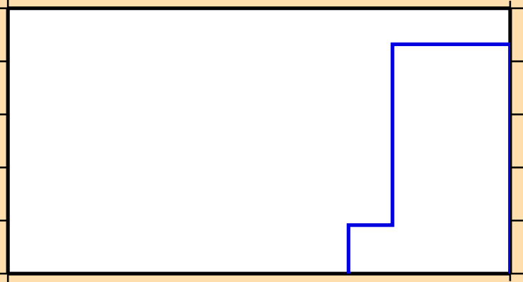
\sigma vs. E for ^{182}\text{Os}(n,2np)
