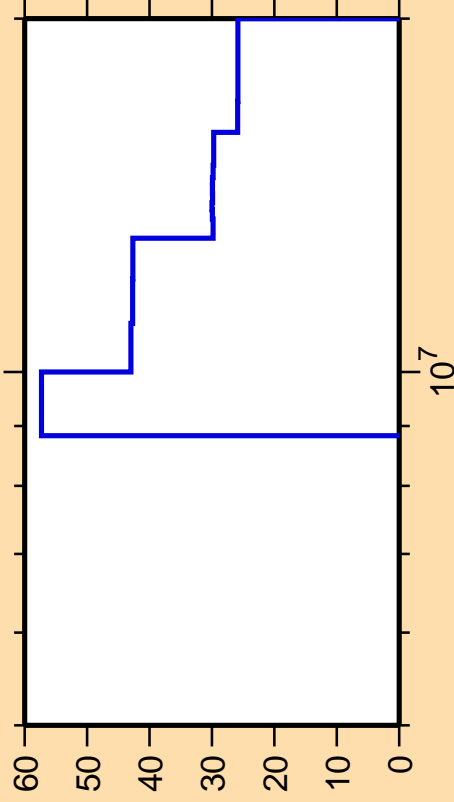
\Delta\sigma/\sigma vs. E for ^{182}\text{Os}(n,2n)
