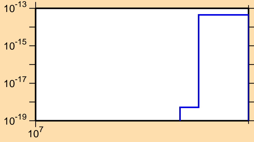
\sigma vs. E for ^{182}\text{Os}(n,3n\alpha)
