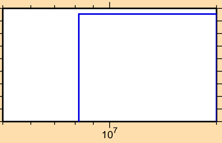
\sigma vs. E for ^{182}\text{Os}(n,2np)
