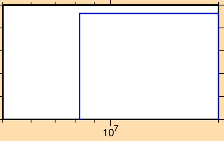
\sigma vs. E for ^{182}\text{Os}(\text{mt117})
