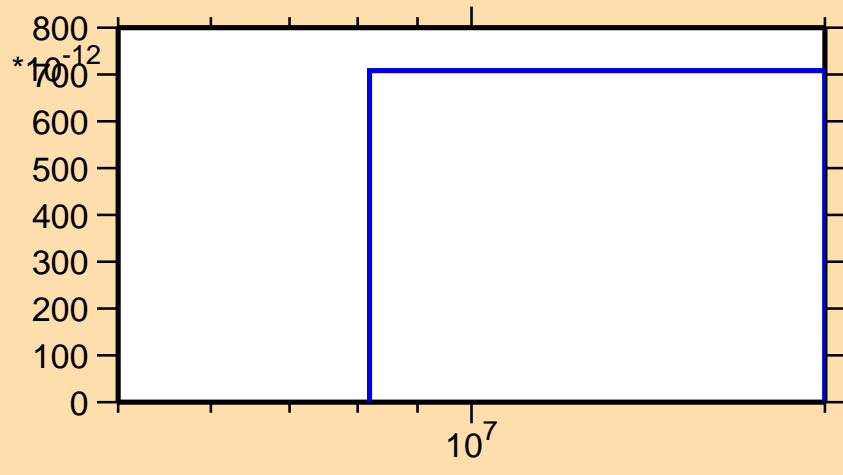
\sigma vs. E for ^{182}\text{Os}(n,\text{He}3)
