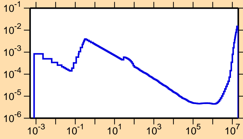
\sigma vs. E for ^{183}\text{Os}(n,\alpha)
