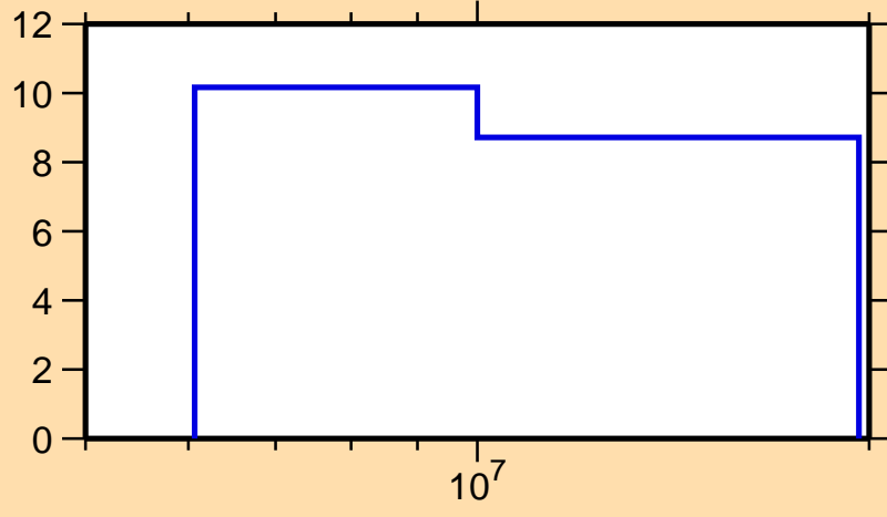
\Delta\sigma/\sigma vs. E for ^{183}\text{Os}(n,\text{nonel.})
