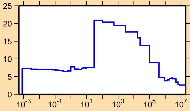
\sigma vs. E for ^{183}\text{Os}(n,\text{el.})
