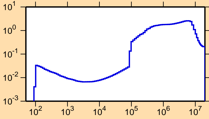
\sigma vs. E for ^{183}\text{Os}(n,\text{inel.})
