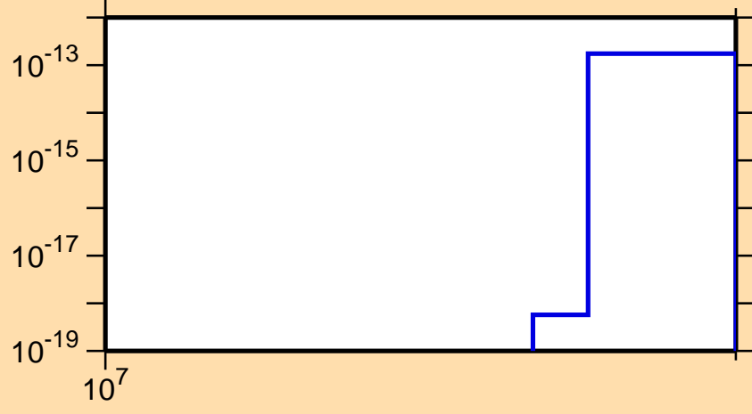
\sigma vs. E for ^{183}\text{Os}(n,3n\alpha)
