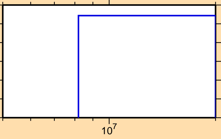
\sigma vs. E for ^{183}\text{Os}(n,2np)
