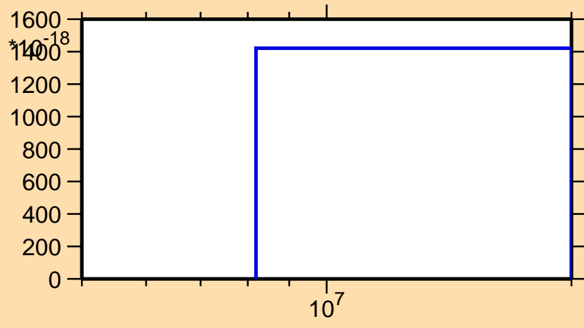
\sigma vs. E for ^{183}\text{Os}(n,3n\alpha)
