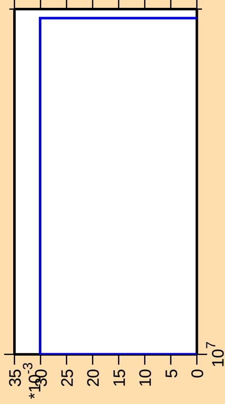
\Delta\sigma/\sigma vs. E for ^{184}\text{Os}(\text{mt } 45)
