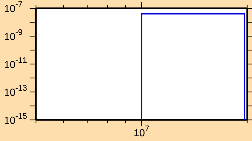
\sigma vs. E for ^{184}\text{Os}(n,2n\alpha)
