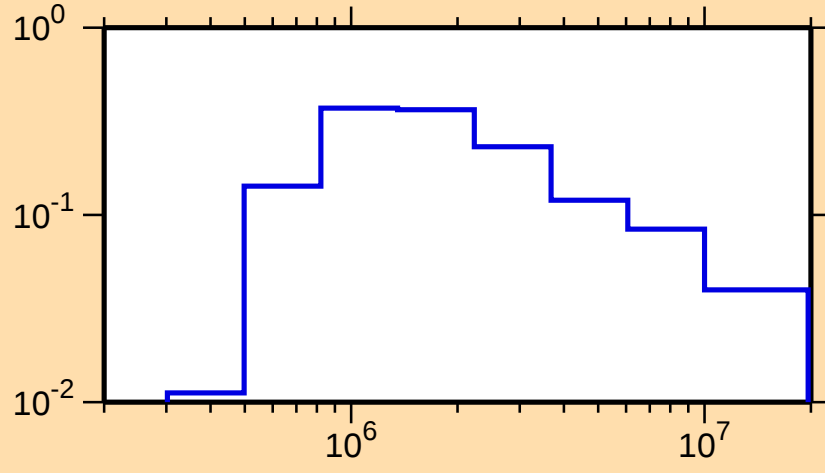
\sigma vs. E for ^{184}\text{Os}(n,n_2)
