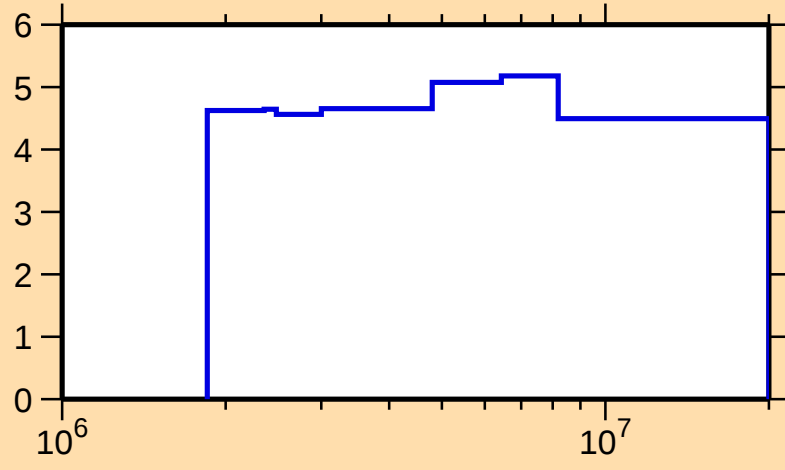
\Delta\sigma/\sigma vs. E for ^{184}\text{Os}(n,n\text{nonel.})
