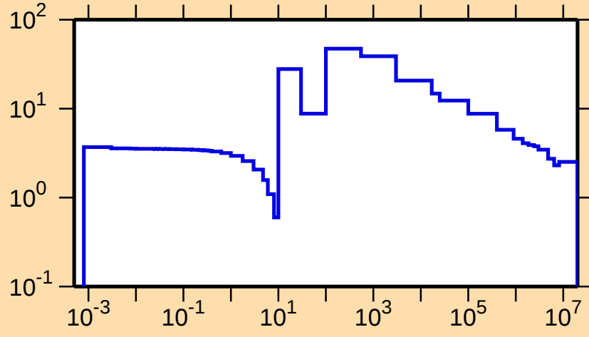
\sigma vs. E for ^{184}\text{Os}(n,\text{el.})
