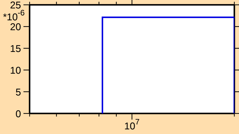
\sigma vs. E for ^{184}\text{Os}(n,t)
