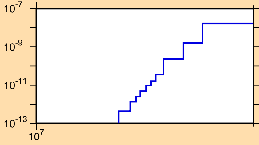
\sigma vs. E for ^{185}\text{Os}(n,\text{He3})
