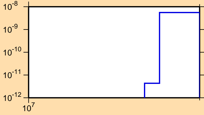
\sigma vs. E for ^{185}\text{Os}(n,nt)
