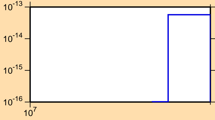
\sigma vs. E for ^{185}\text{Os}(n,\text{pt})
