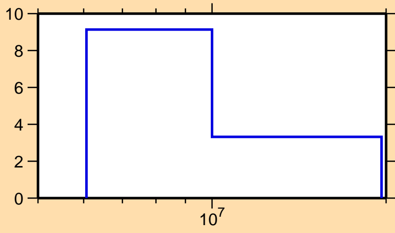
\Delta\sigma/\sigma vs. E for ^{185}\text{Os}(n,\text{tot.})
