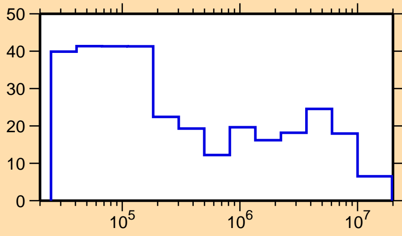
\Delta\sigma/\sigma vs. E for ^{185}\text{Os}(n,\text{el.})
