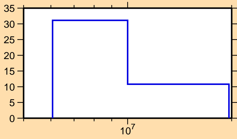
\Delta\sigma/\sigma vs. E for ^{185}\text{Os}(n,2n)
