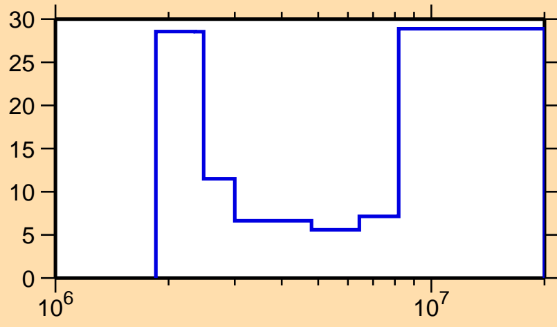
\Delta\sigma/\sigma vs. E for ^{186}\text{Os}(n,n\text{cont.})
