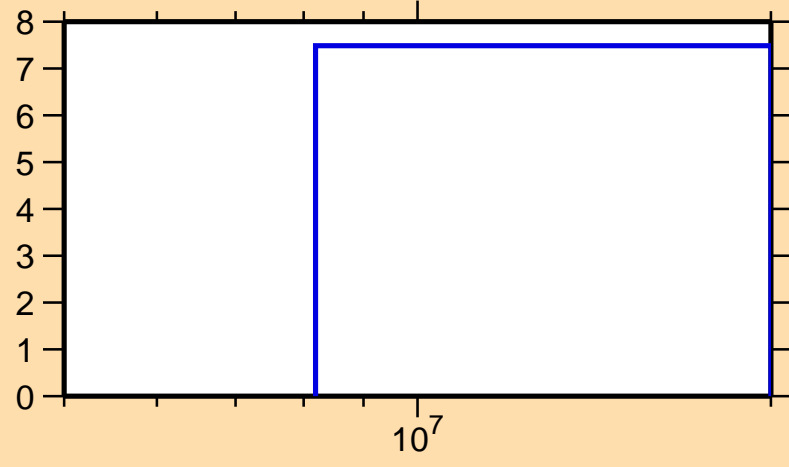
\Delta\sigma/\sigma vs. E for ^{186}\text{Os}(n,2n)
