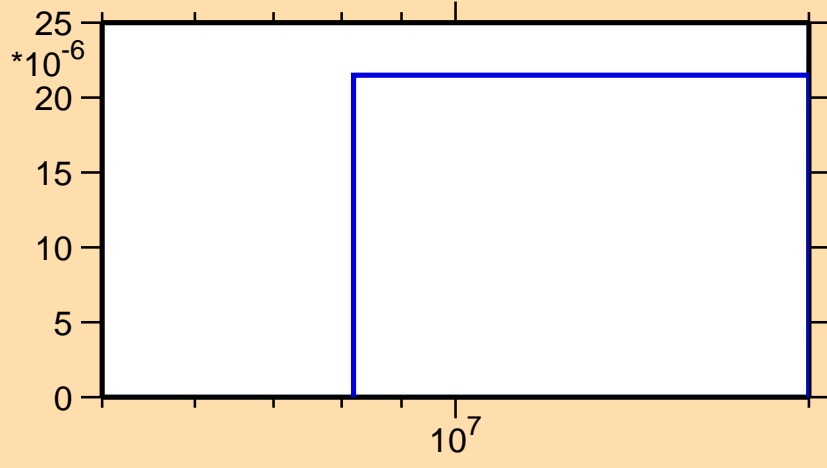
\sigma vs. E for ^{186}\text{Os}(n,t)
