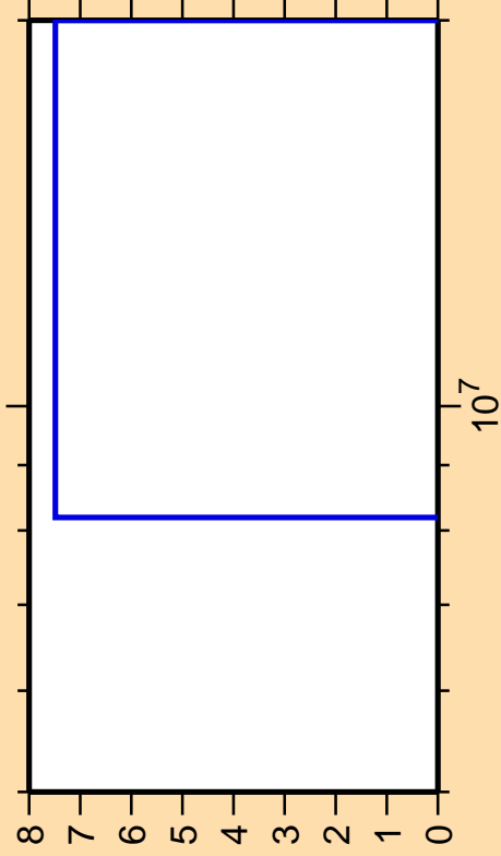
\Delta\sigma/\sigma vs. E for ^{186}\text{Os}(n,2n)
