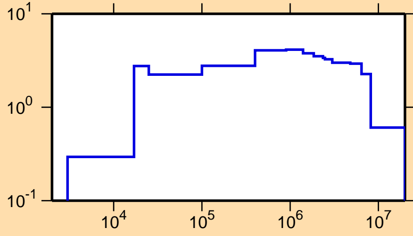
\sigma vs. E for ^{187}\text{Os}(n,\text{inel.})
