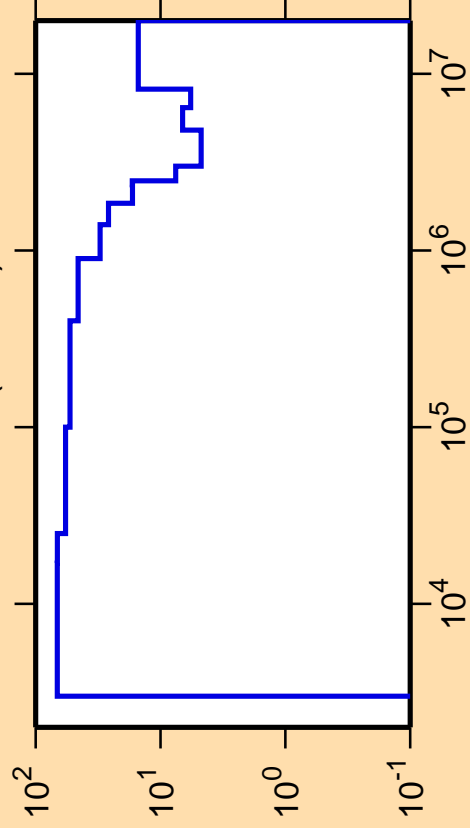
\Delta\sigma/\sigma vs. E for ^{187}\text{Os}(n,\text{inel.})
