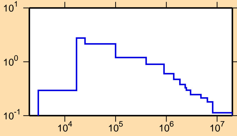
\sigma vs. E for ^{187}\text{Os}(n,n_1)
