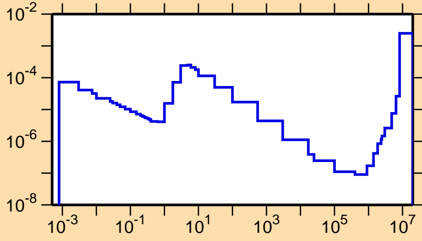
\sigma vs. E for ^{187}\text{Os}(n,\alpha)
