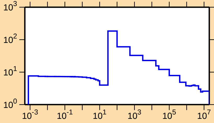
\sigma vs. E for ^{188}\text{Os}(n,\text{el.})
