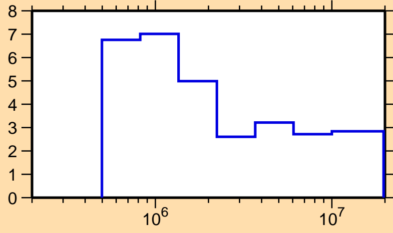
\Delta\sigma/\sigma vs. E for ^{189}\text{Os}(n,\text{tot.})
