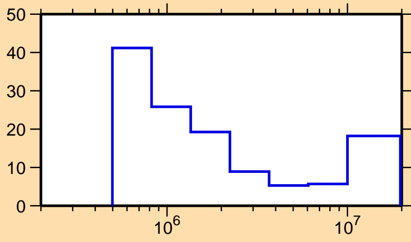
\Delta\sigma/\sigma vs. E for ^{189}\text{Os}(n,n\text{cont.})
