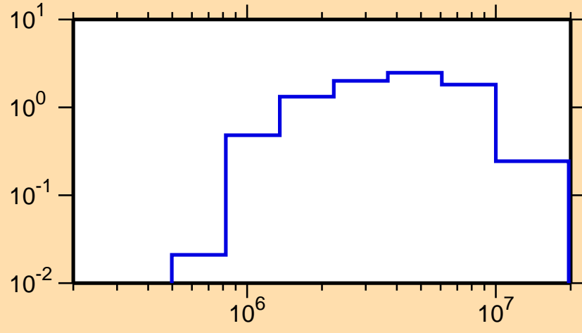
\sigma vs. E for ^{189}\text{Os}(n,n\text{cont.})
