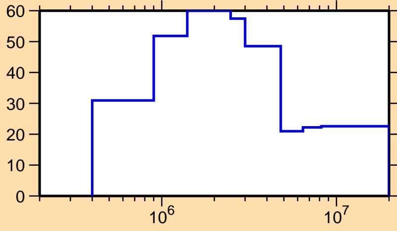
\Delta\sigma/\sigma vs. E for ^{189}\text{Os}(n,n_1)
