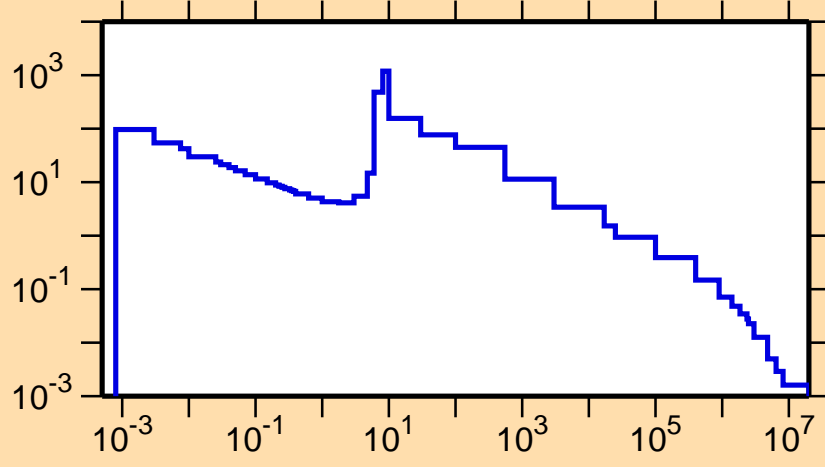
\sigma vs. E for ^{189}\text{Os}(n,\gamma)
