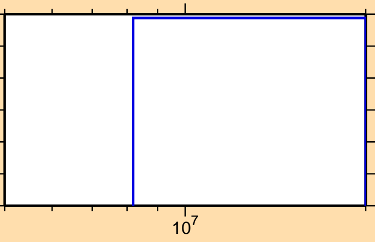
\sigma vs. E for ^{189}\text{Os} (mt 11)
