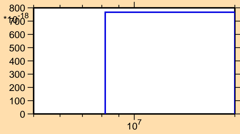
\sigma vs. E for ^{189}\text{Os}(n,3n\alpha)
